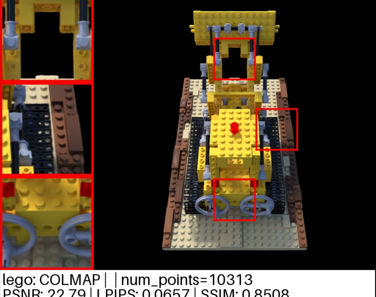
lego: COLMAP | | num_points=10313 PSNR: 22.79 | LPIPS: 0.0657 | SSIM: 0.8508
