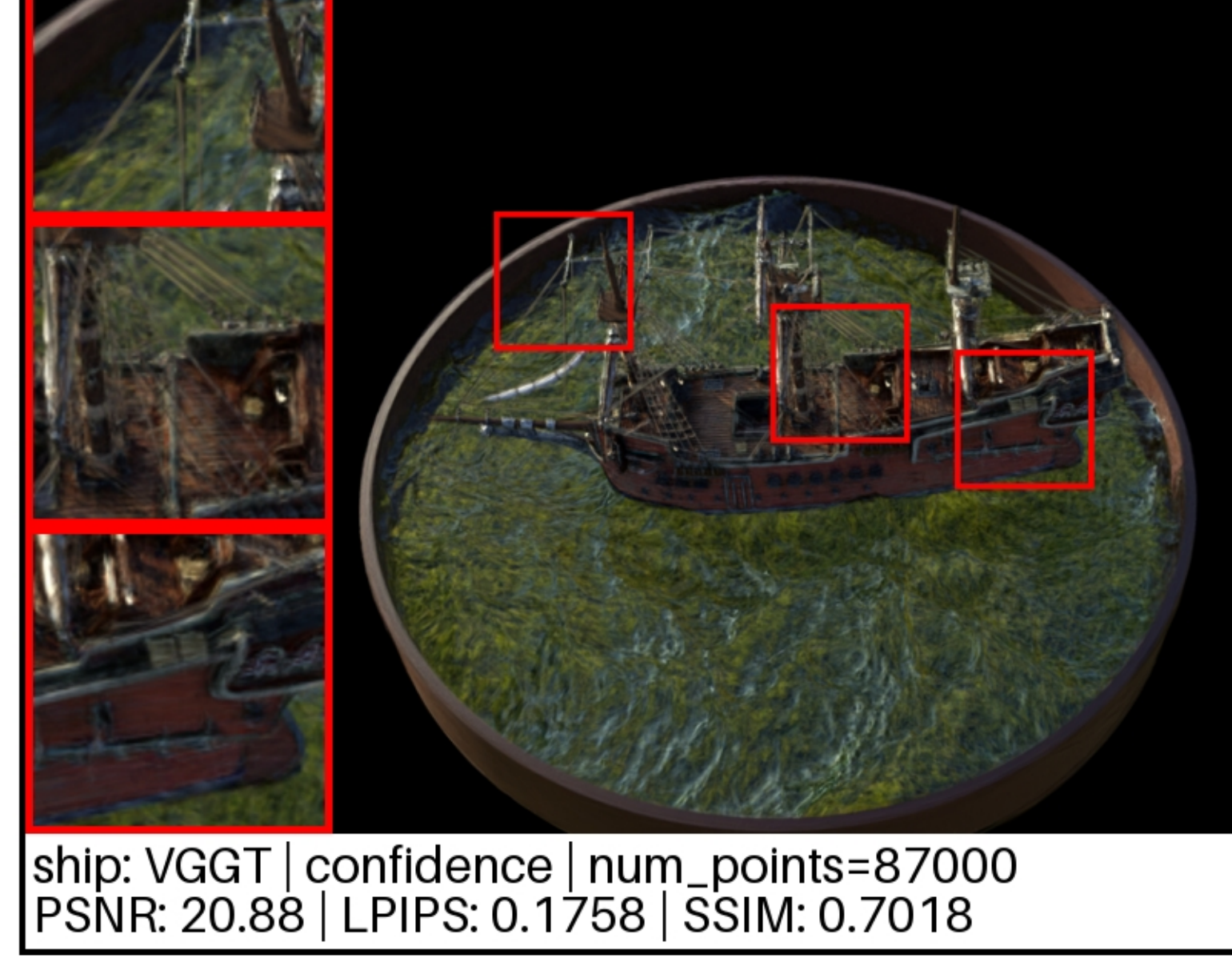
ship: VGGT | confidence | num_points=87000 PSNR: 20.88 | LPIPS: 0.1758 | SSIM: 0.7018
