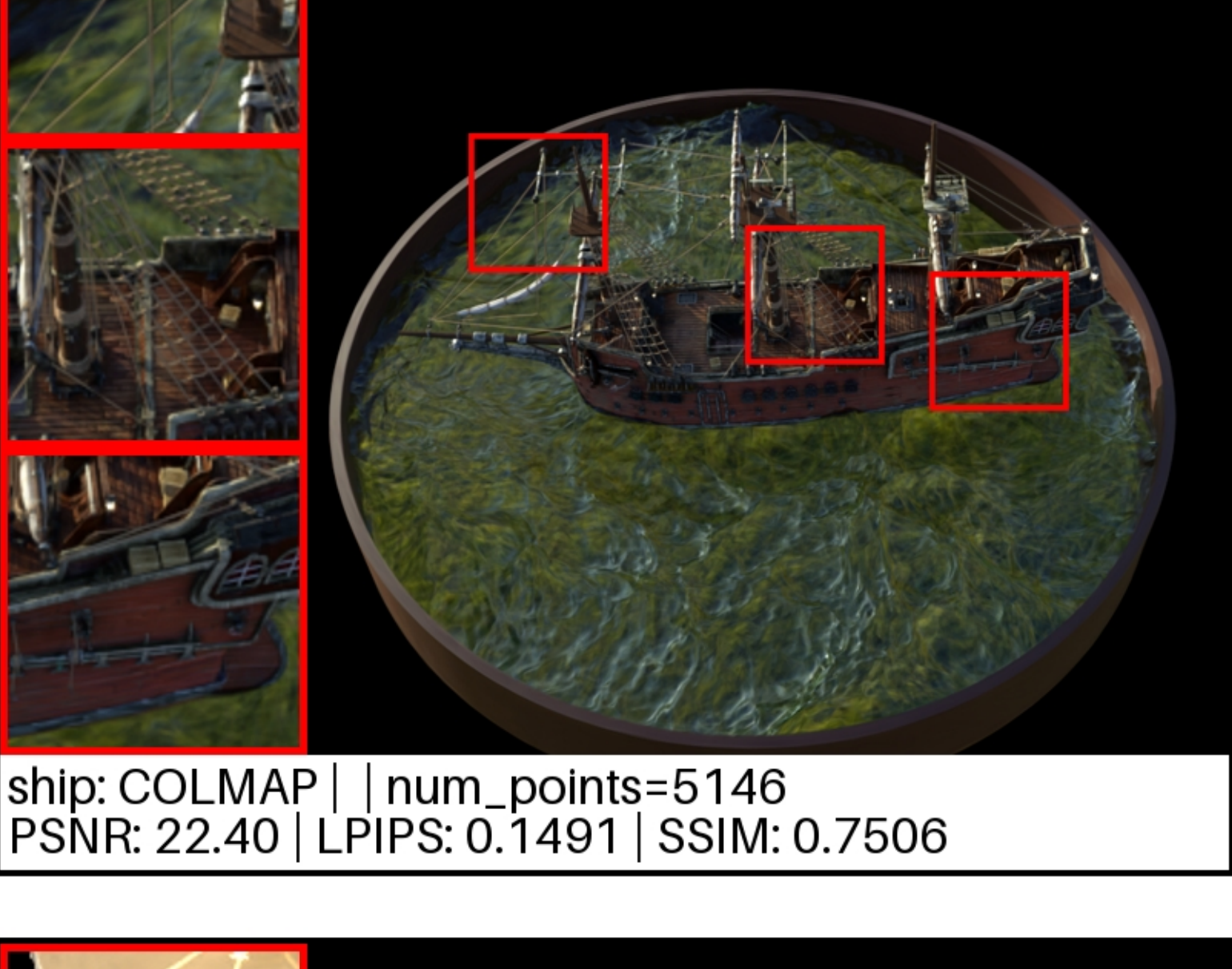
ship: COLMAP | | num_points=5146 PSNR: 22.40 | LPIPS: 0.1491 | SSIM: 0.7506
