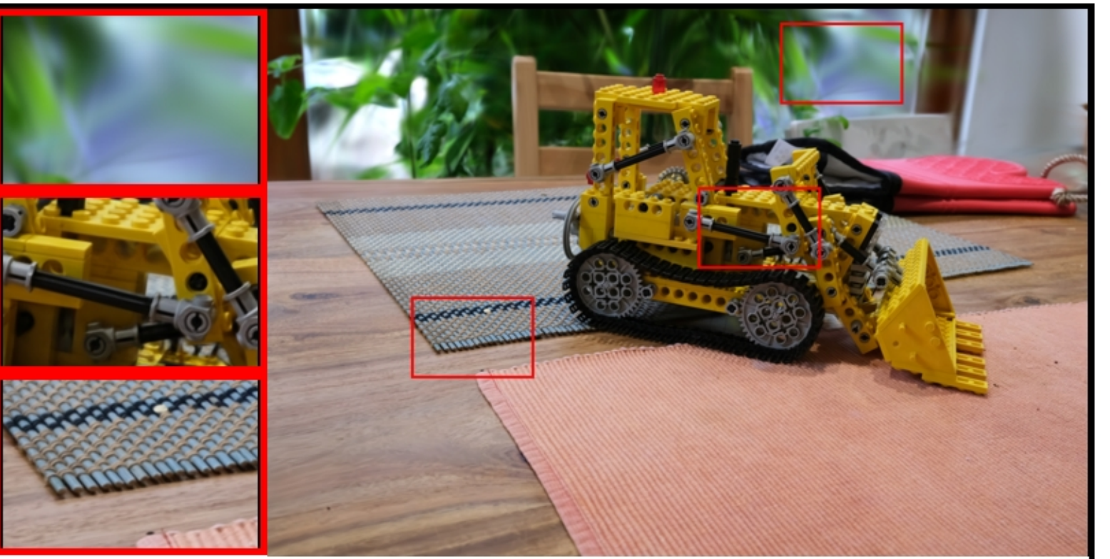
kitchen: COLMAP | Pose Opt PSNR: 22.44 | LPIPS: 0.1272 | SSIM: 0.5514
