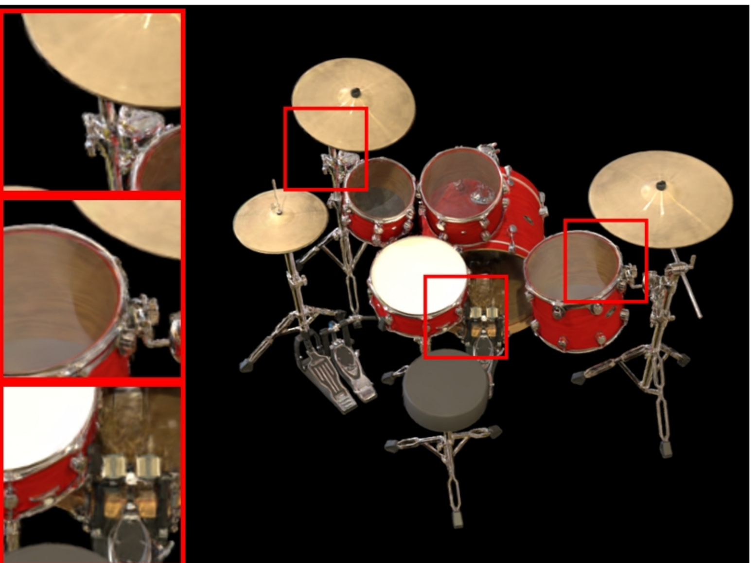
drums: VGGT | PSNR: 19.67 | LPIPS: 0.1061 | SSIM: 0.8356
