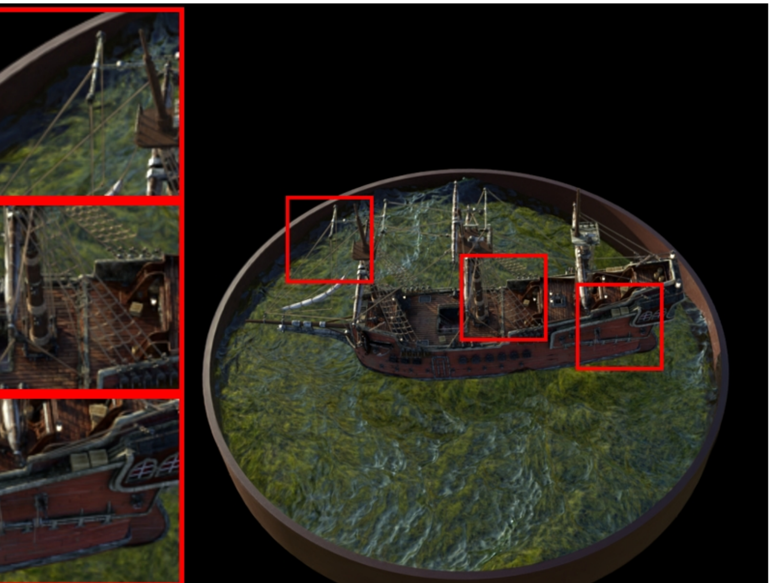
ship: VGGT | Pose Opt PSNR: 22.86 | LPIPS: 0.1296 | SSIM: 0.7485
