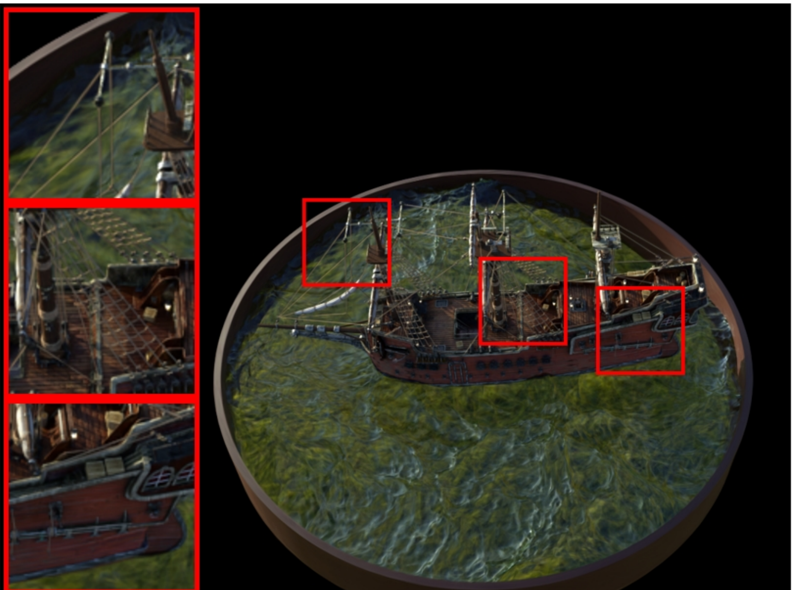
ship: COLMAP | PSNR: 22.40 | LPIPS: 0.1491 | SSIM: 0.7506
