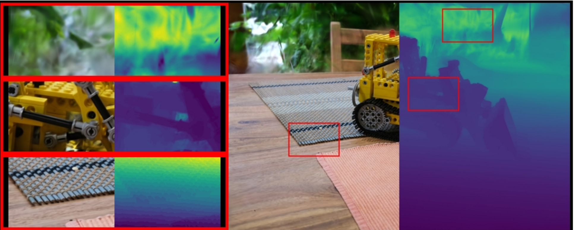
kitchen: VGGT | Standard | full PSNR: 20.46 | LPIPS: 0.1884 | SSIM: 0.5392
