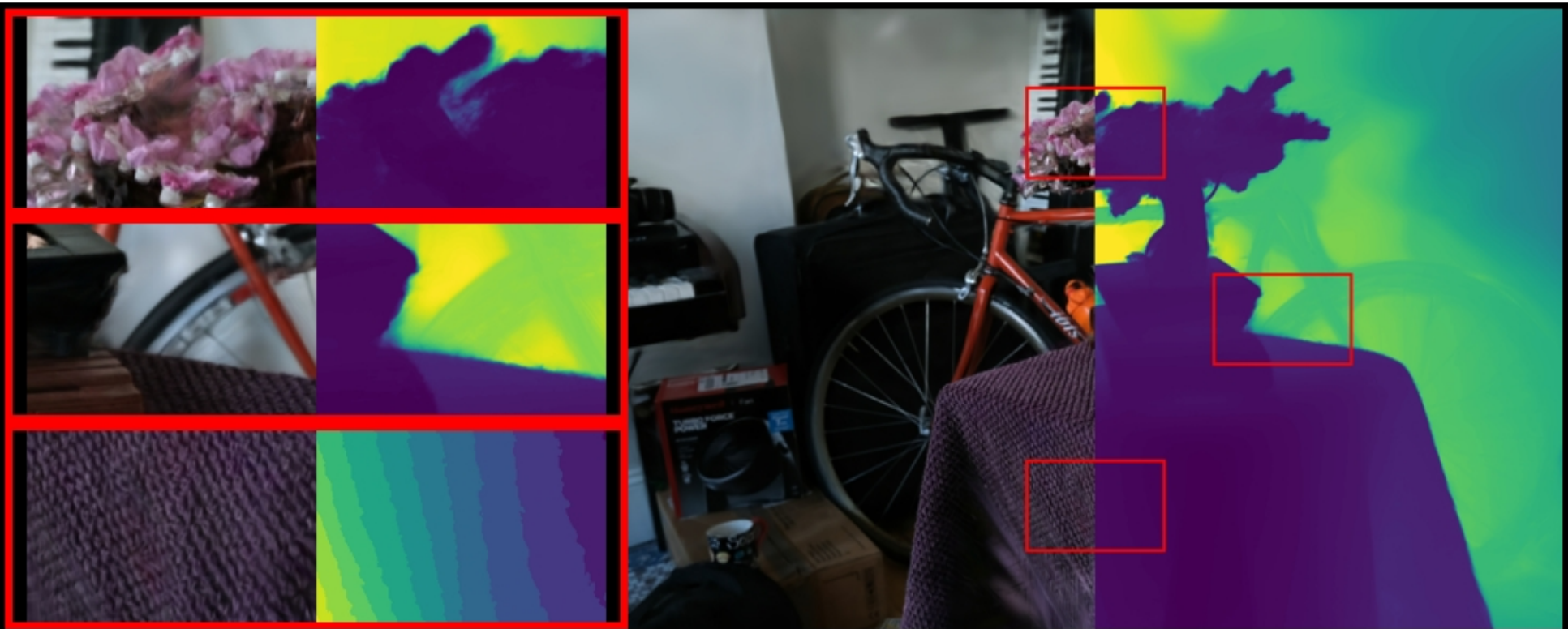
bonsai: VGGT | Standard Shifted | full PSNR: 18.34 | LPIPS: 0.3447 | SSIM: 0.5810
