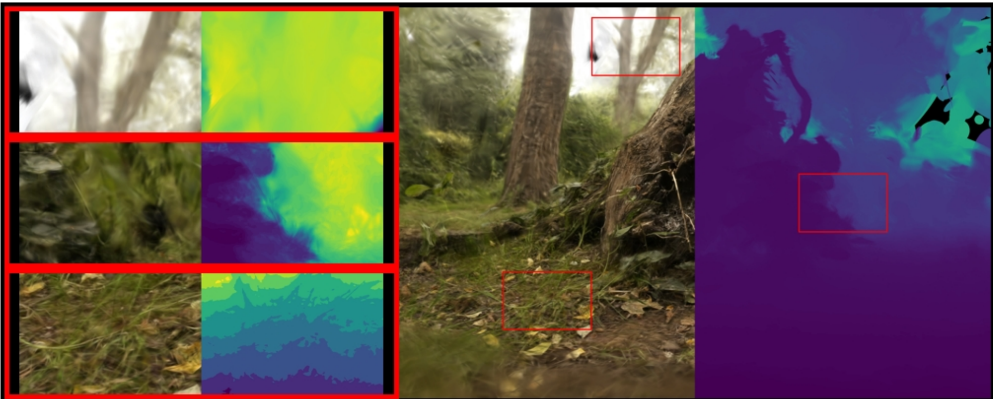
stump: VGGT | Standard | full PSNR: 18.42 | LPIPS: 0.5195 | SSIM: 0.4094
