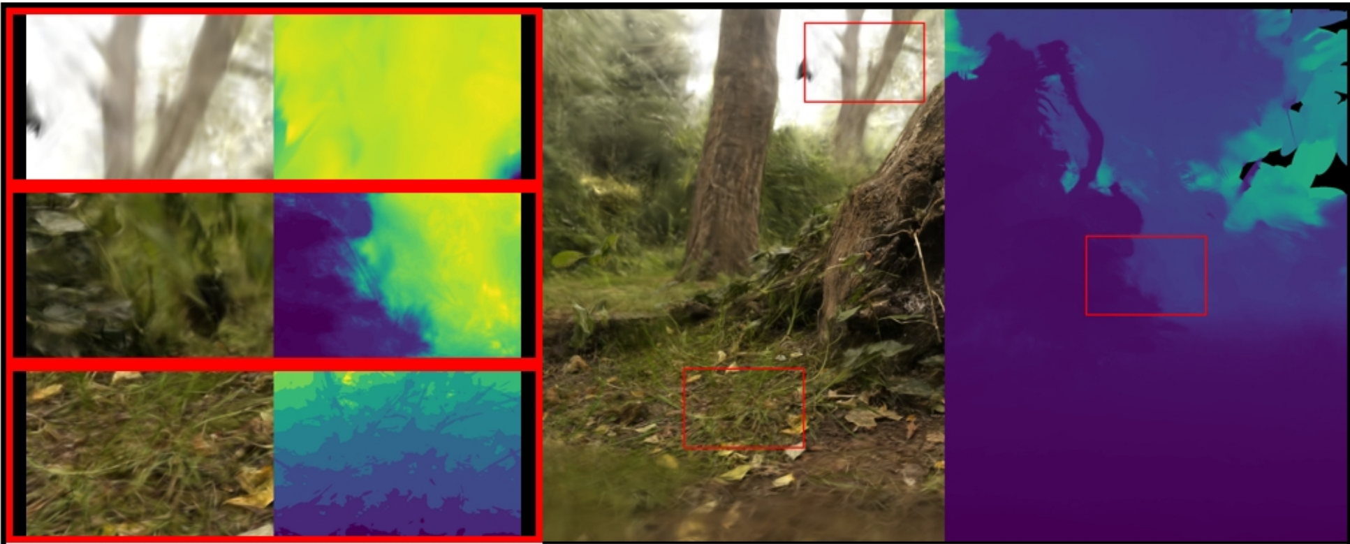
stump: VGGT | | full PSNR: 18.41 | LPIPS: 0.5148 | SSIM: 0.4076
