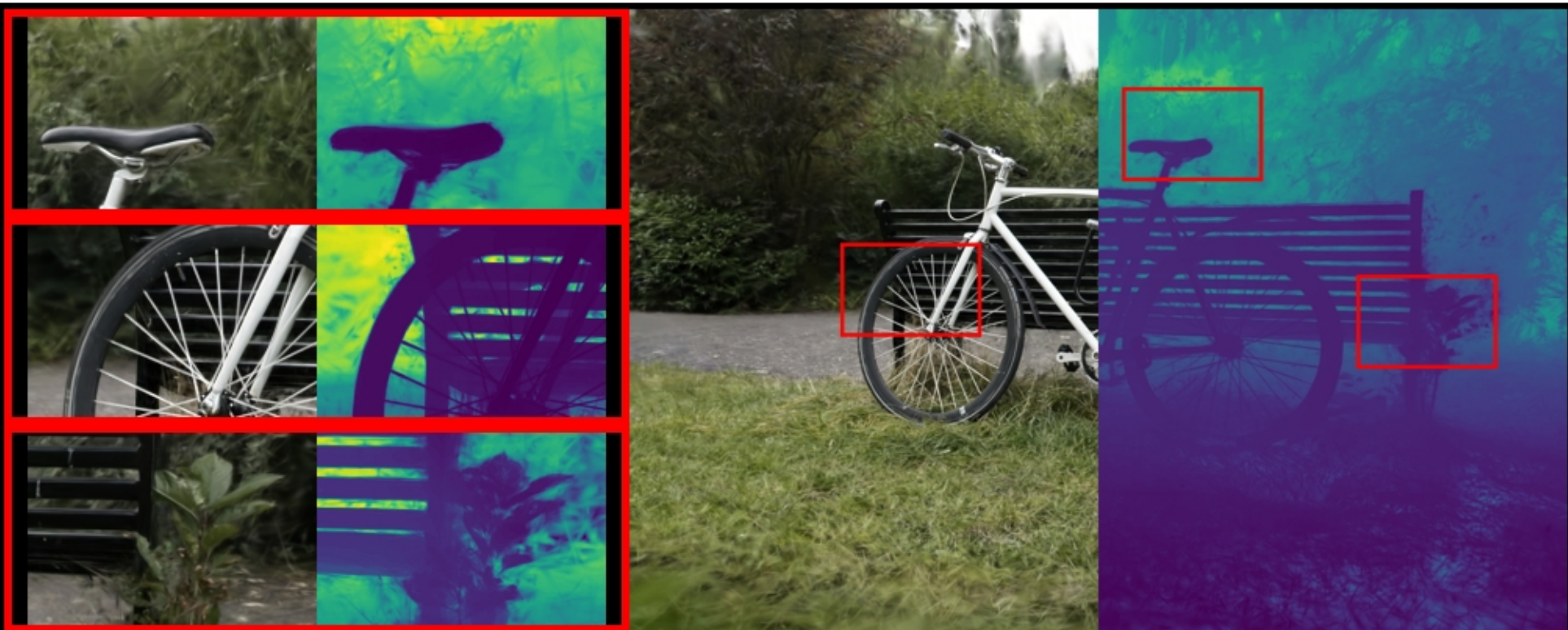
bicycle: VGGT | depth_lambda=0.0 PSNR: 17.38 | LPIPS: 0.3378 | SSIM: 0.2679
