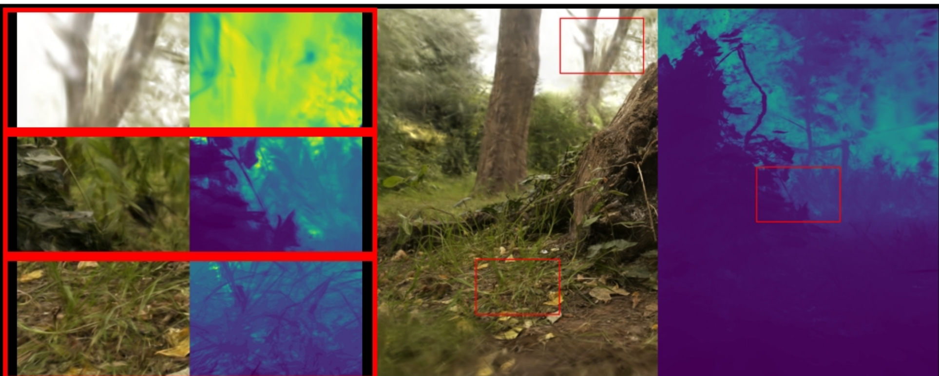
stump: VGGT | depth_lambda=0.0 PSNR: 18.29 | LPIPS: 0.4925 | SSIM: 0.3980
