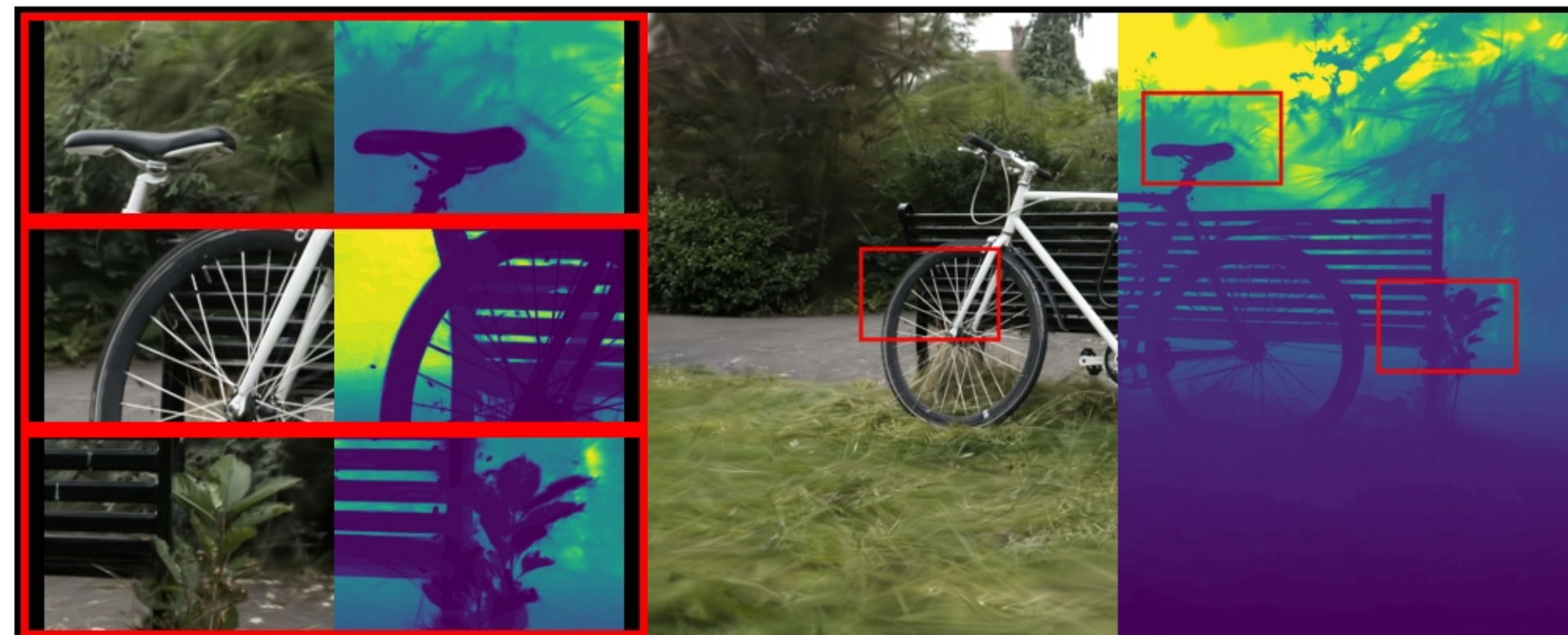
bicycle: COLMAP | points PSNR: 21.66 | LPIPS: 0.3919 | SSIM: 0.5051
