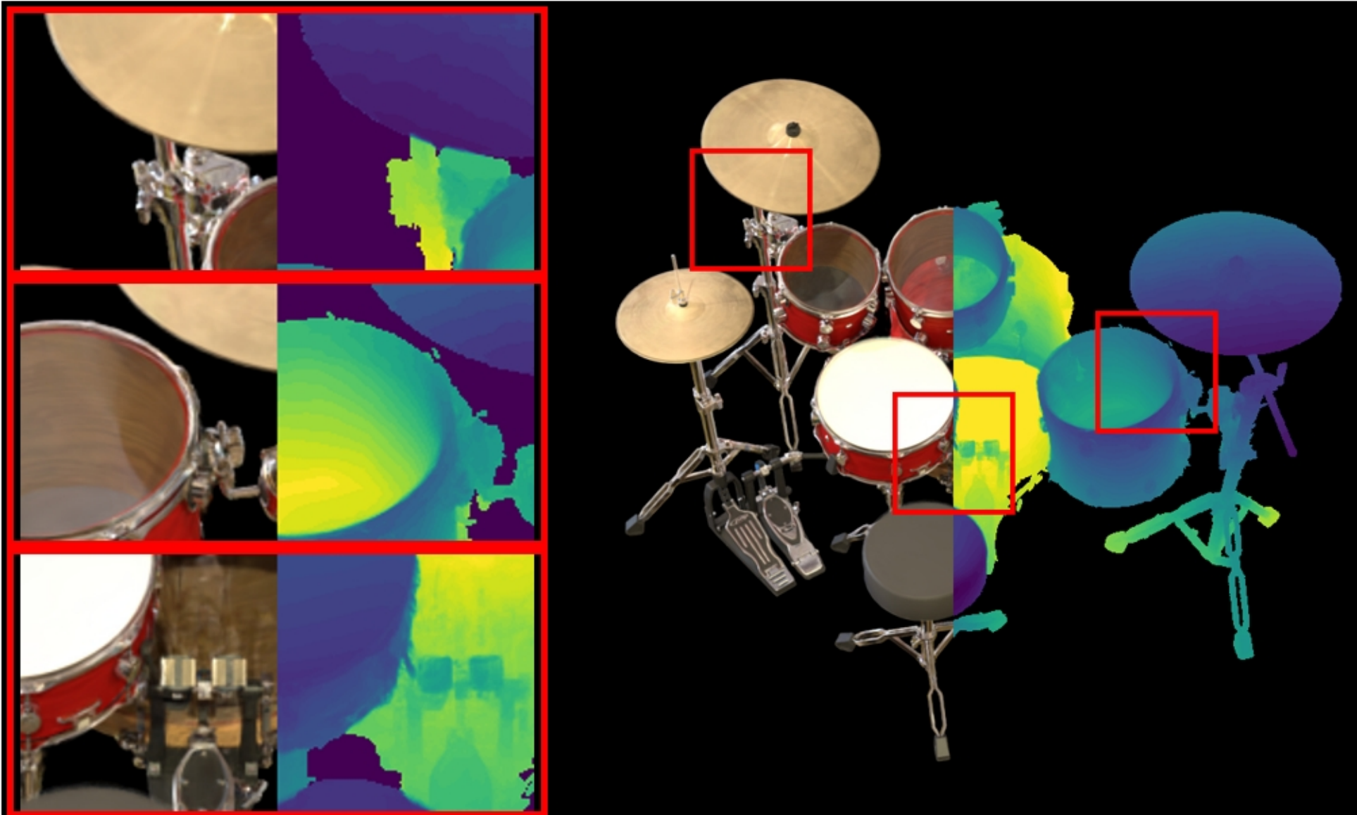
drums: VGGT | closer PSNR: 20.03 | LPIPS: 0.0915 | SSIM: 0.8510
