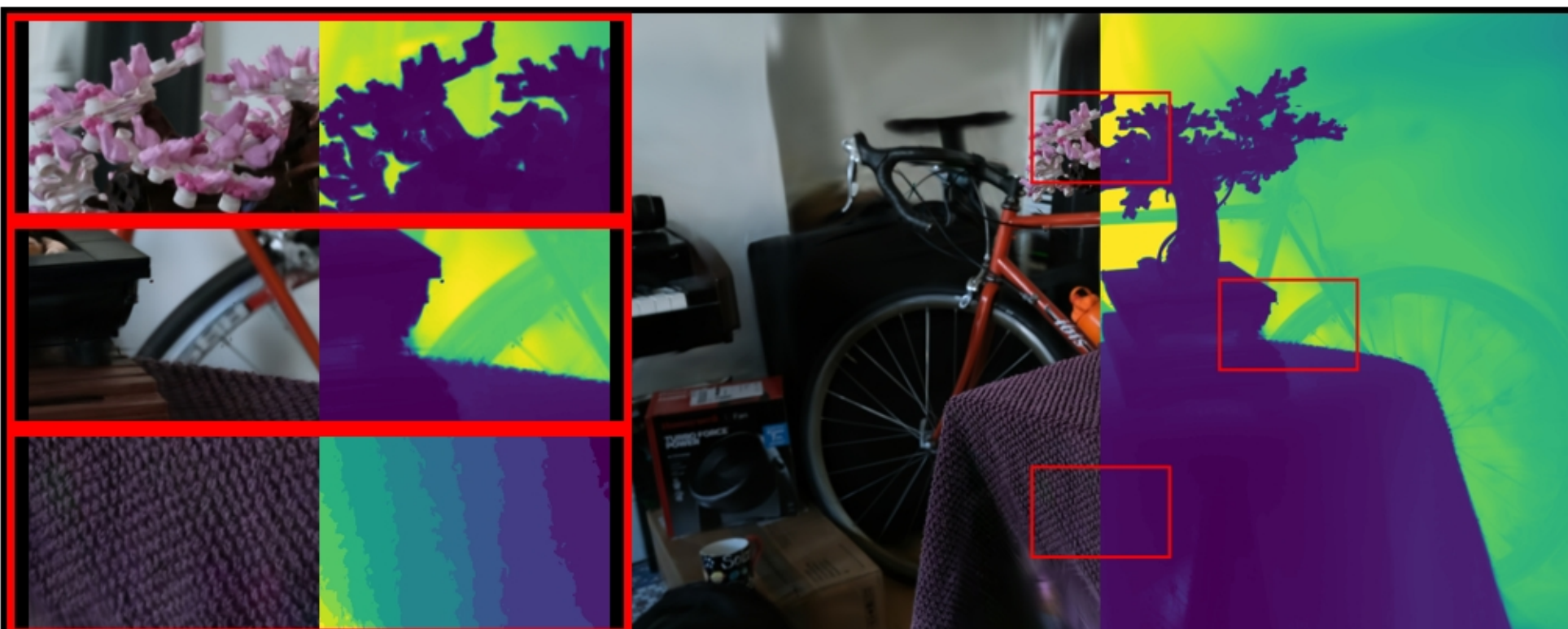
bonsai: COLMAP | points PSNR: 26.08 | LPIPS: 0.1451 | SSIM: 0.8146
