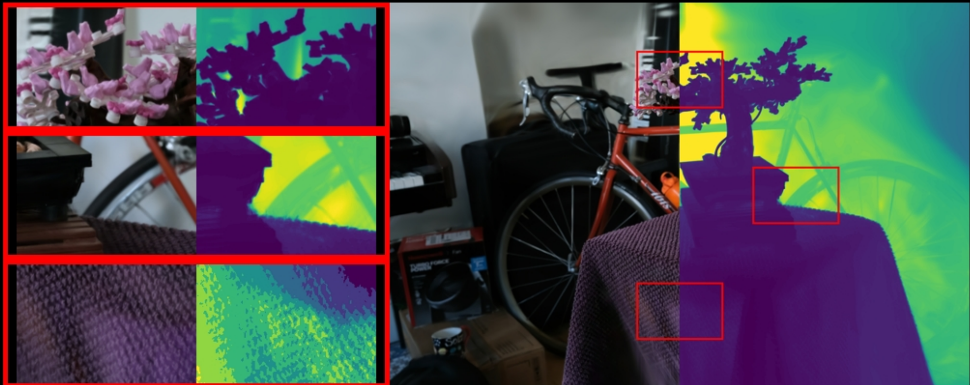
bonsai: COLMAP | PSNR: 25.54 | LPIPS: 0.1440 | SSIM: 0.7955
