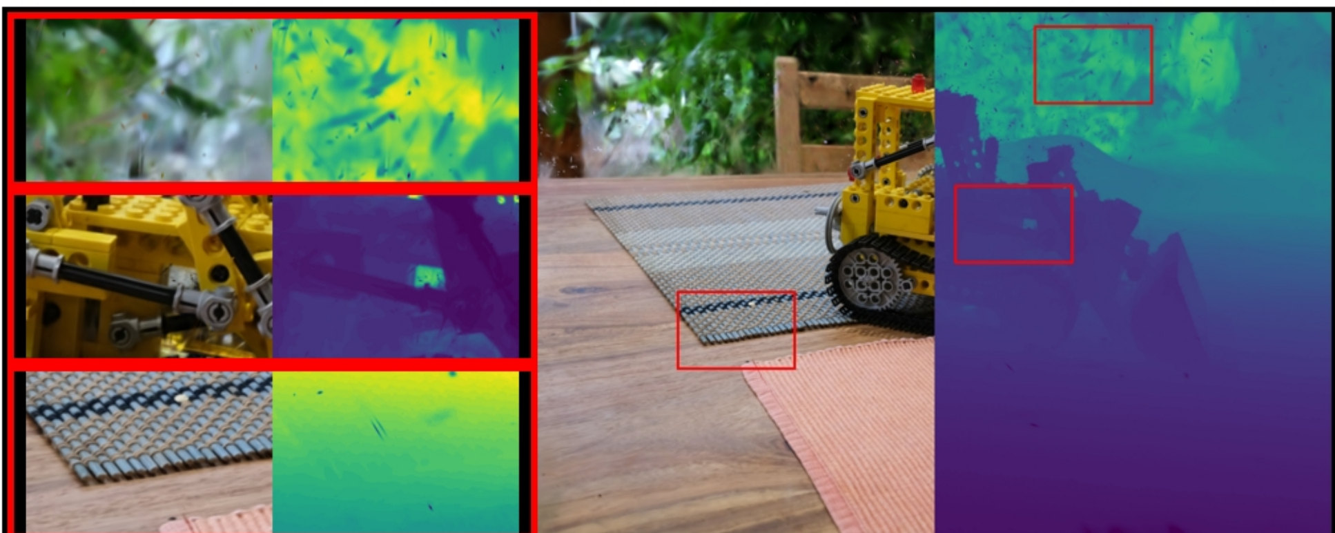
kitchen: VGGT | points PSNR: 20.50 | LPIPS: 0.1977 | SSIM: 0.4960
