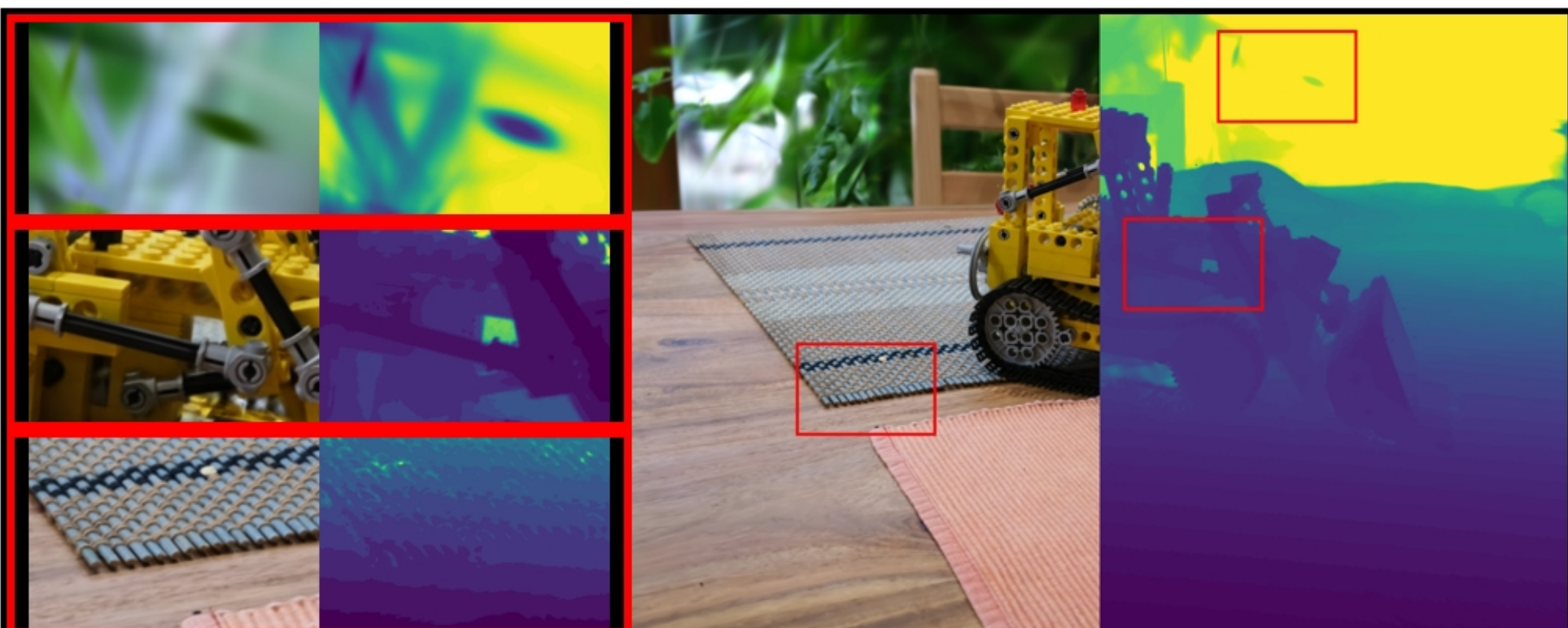
kitchen: COLMAP | points PSNR: 22.30 | LPIPS: 0.1354 | SSIM: 0.5440
