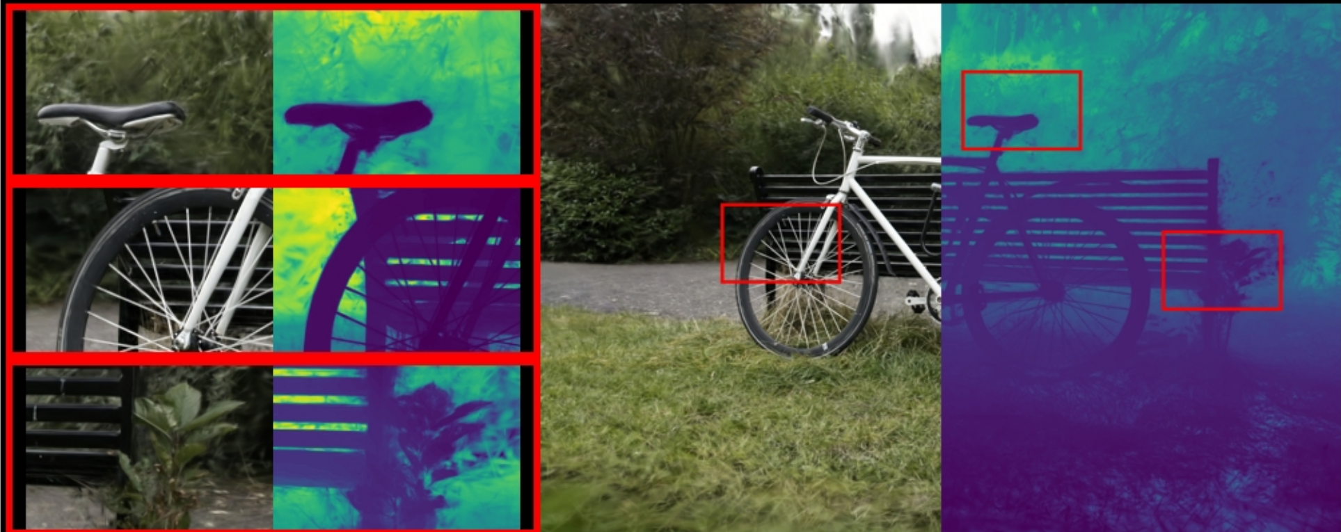
bicycle: VGGT | PSNR: 17.38 | LPIPS: 0.3378 | SSIM: 0.2679
