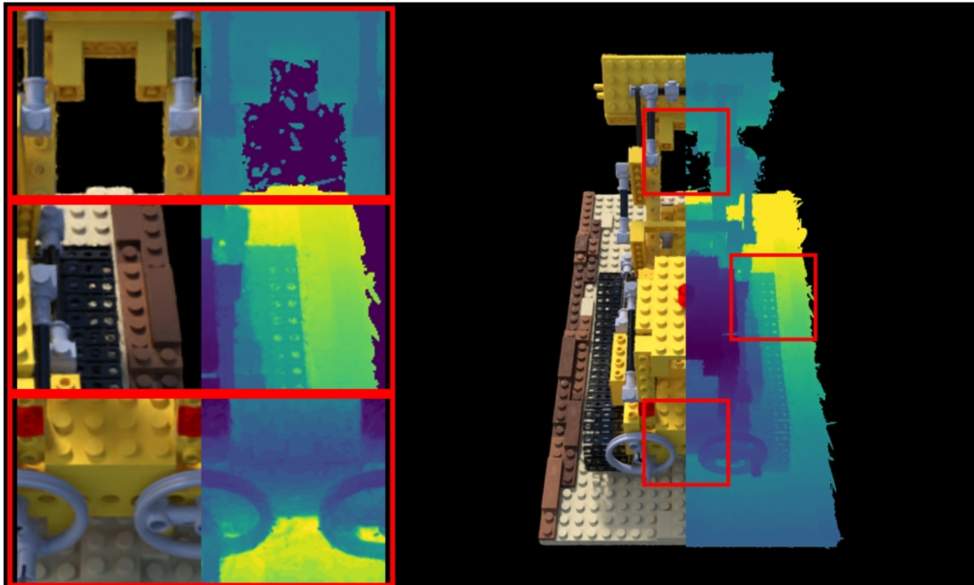
lego: VGGT | points PSNR: 21.99 | LPIPS: 0.0653 | SSIM: 0.8123
