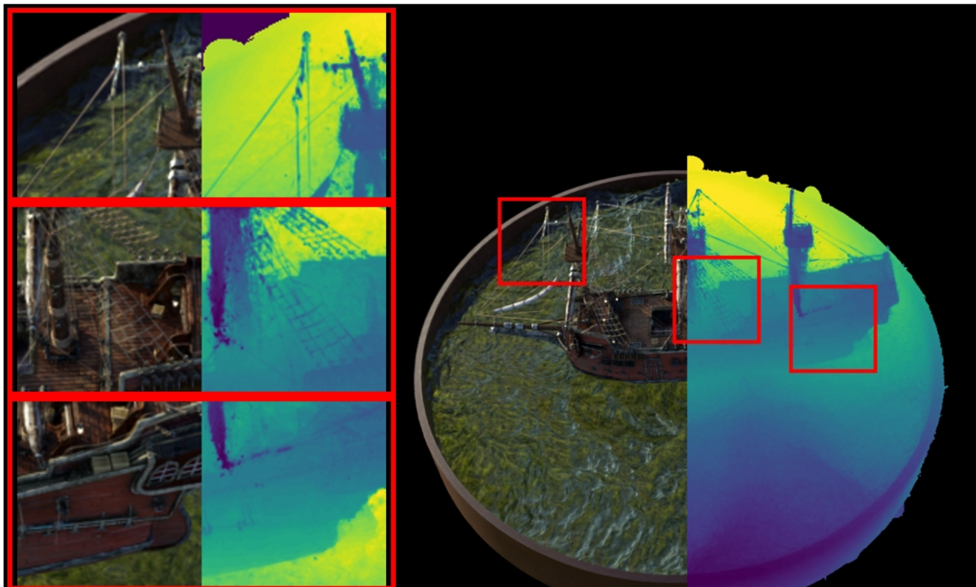
ship: VGGT | points PSNR: 23.51 | LPIPS: 0.1262 | SSIM: 0.7634
