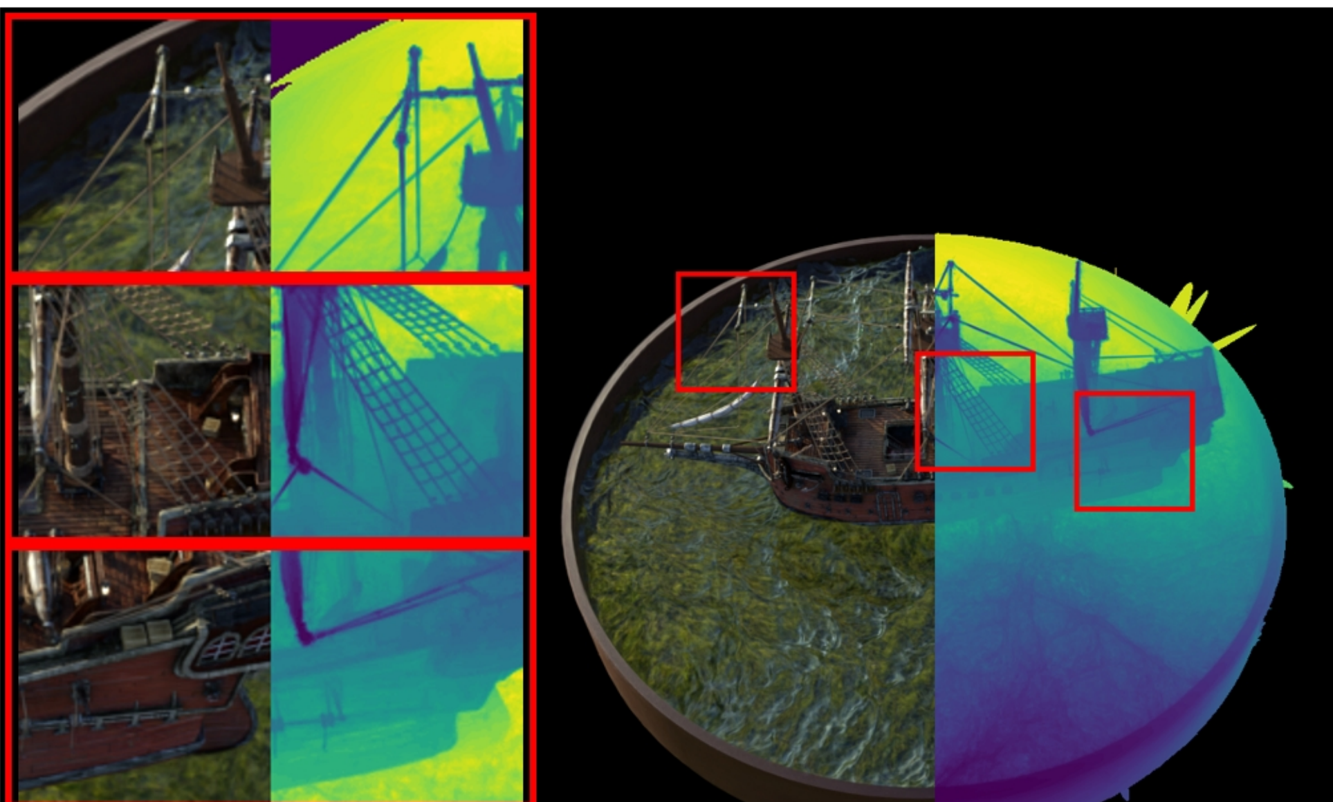
ship: VGGT | PSNR: 22.86 | LPIPS: 0.1296 | SSIM: 0.7485
