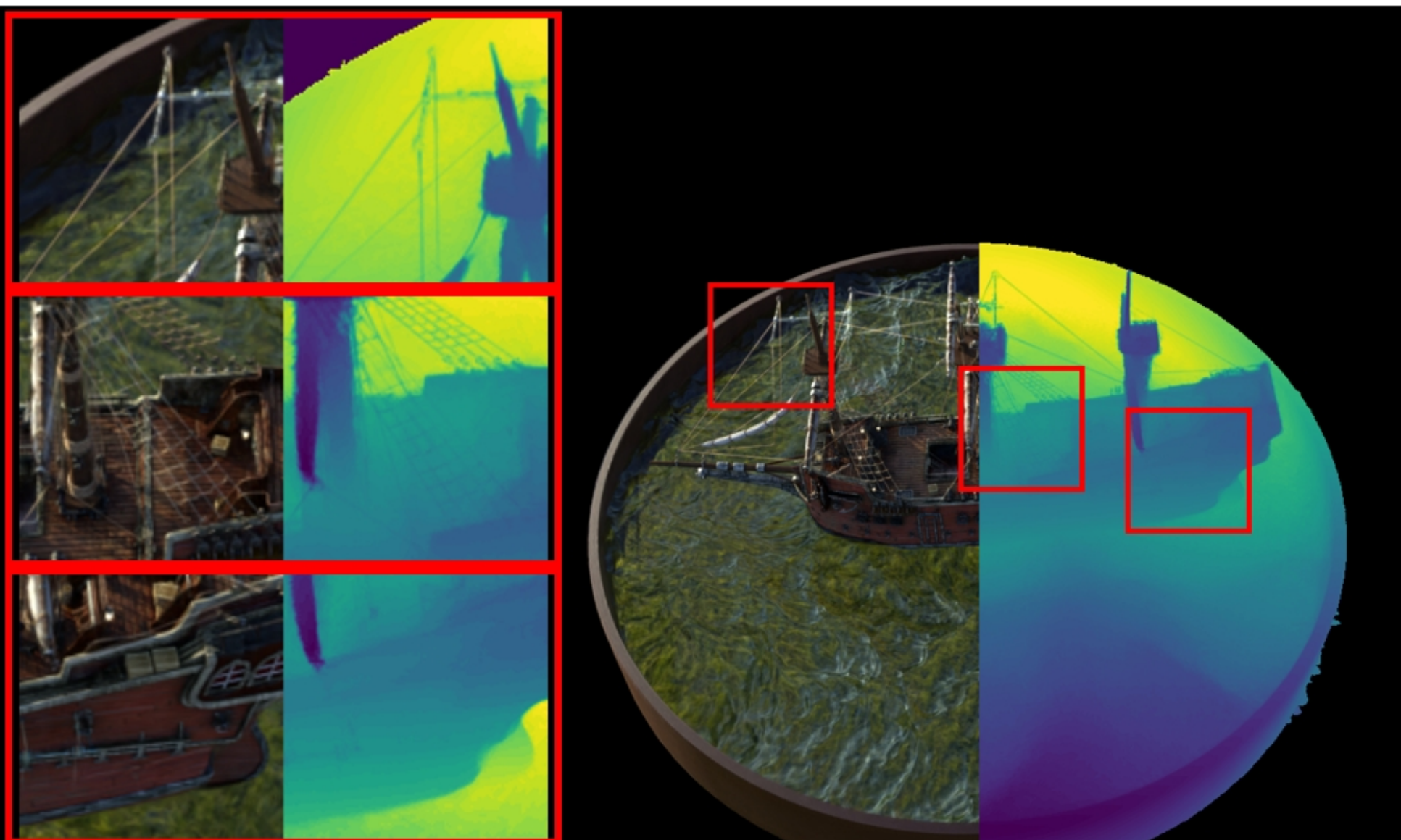
ship: VGGT | full PSNR: 23.49 | LPIPS: 0.1317 | SSIM: 0.7647
