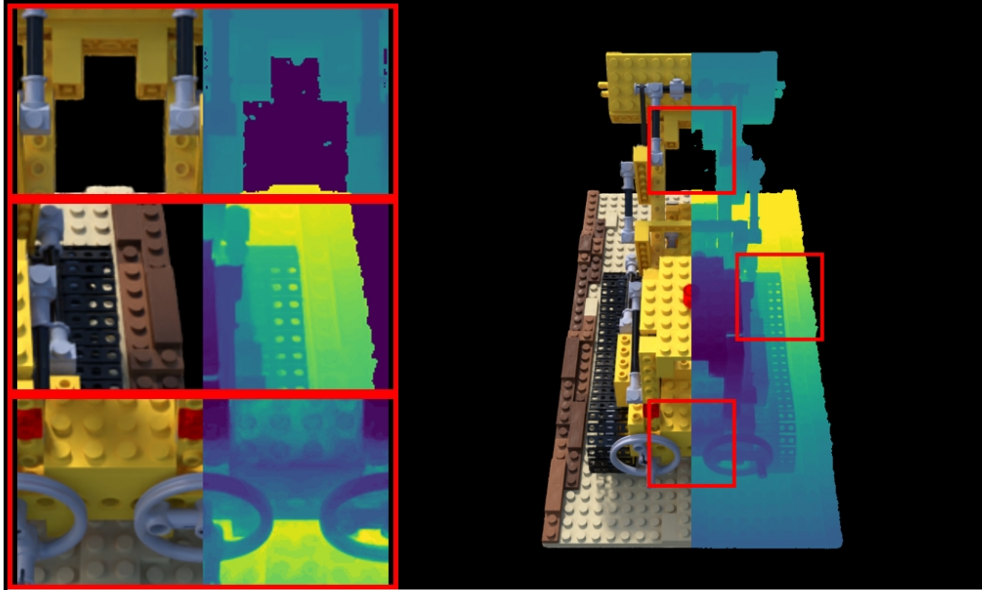
lego: VGGT | closer PSNR: 20.37 | LPIPS: 0.0786 | SSIM: 0.7747
