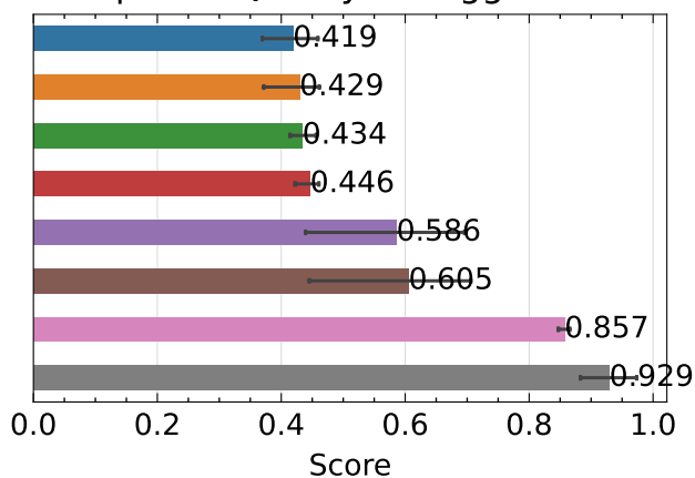
Composite Quality ↑ - vggg - indoor
