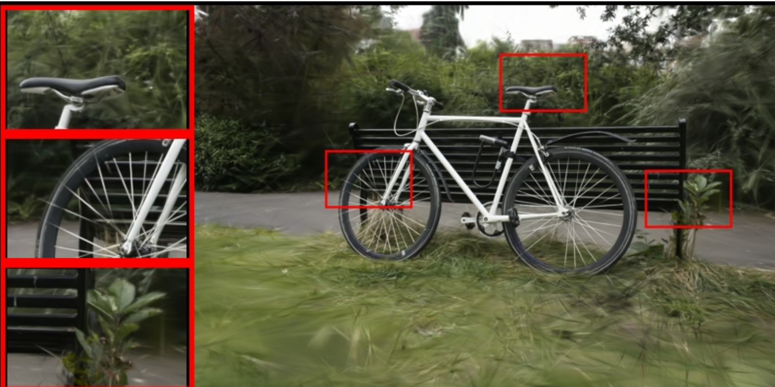
bicycle: COLMAP | Random Init PSNR: 21.16 | LPIPS: 0.5056 | SSIM: 0.4540
