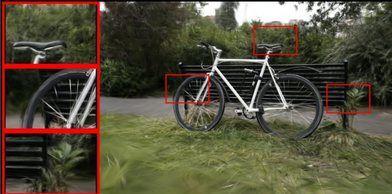
bicycle: VGGT | Random Init | Use BA PSNR: 17.71 | LPIPS: 0.5619 | SSIM: 0.3046
