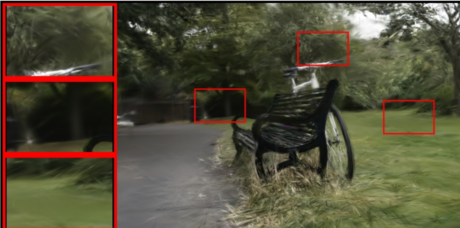
bicycle: VGGT | Random Init PSNR: 17.86 | LPIPS: 0.5818 | SSIM: 0.3078
