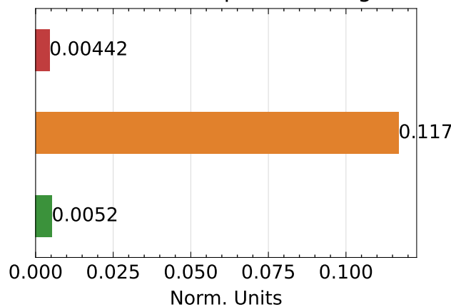
Validation Step RTE ↓ - ship
