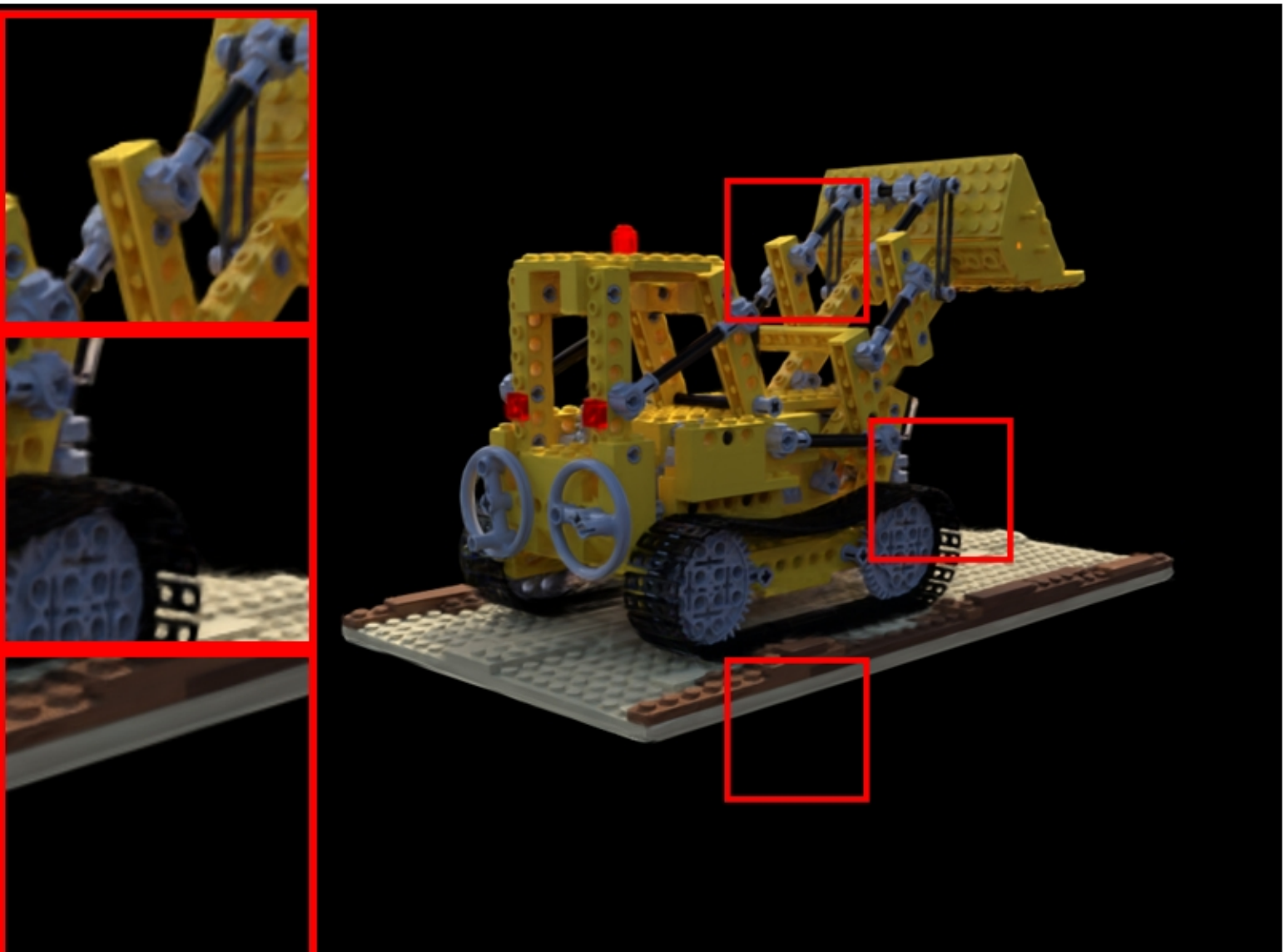
lego: VGGT | Random Init PSNR: 20.55 | LPIPS: 0.1072 | SSIM: 0.7763
