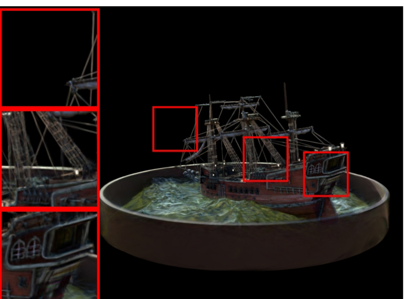
ship: VGGT | Random Init PSNR: 20.87 | LPIPS: 0.2035 | SSIM: 0.7150
