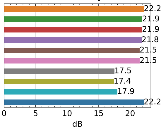
PSNR ↑ - bicycle
