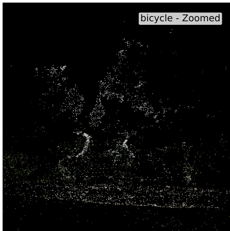
COLMAP | | |
