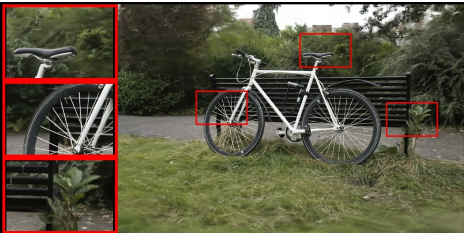
bicycle: COLMAP | | PSNR: 22.16 | LPIPS: 0.3495 | SSIM: 0.5587
