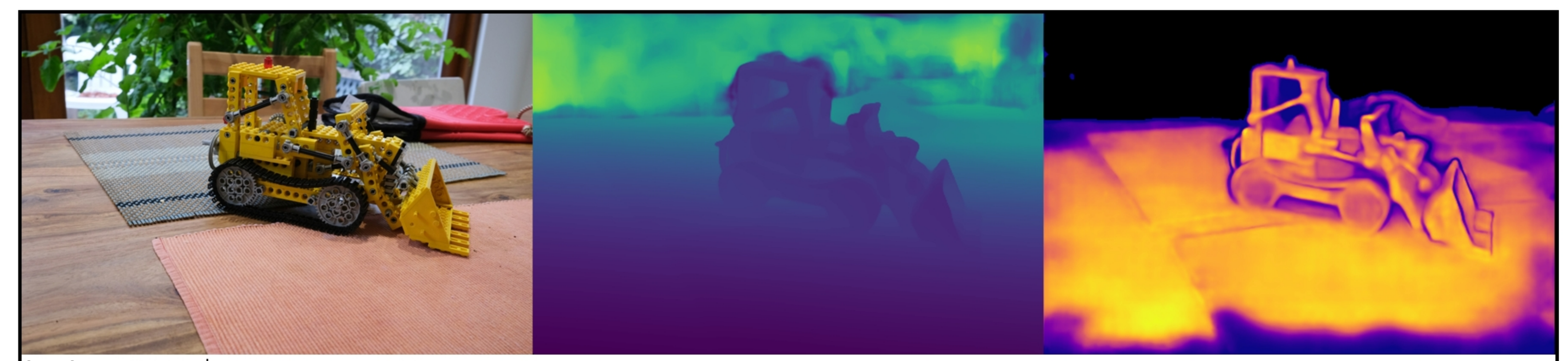
kitchen: VGGT | num_images=70 Original | Depth (max=2.39) | Confidence (max=31.91)
