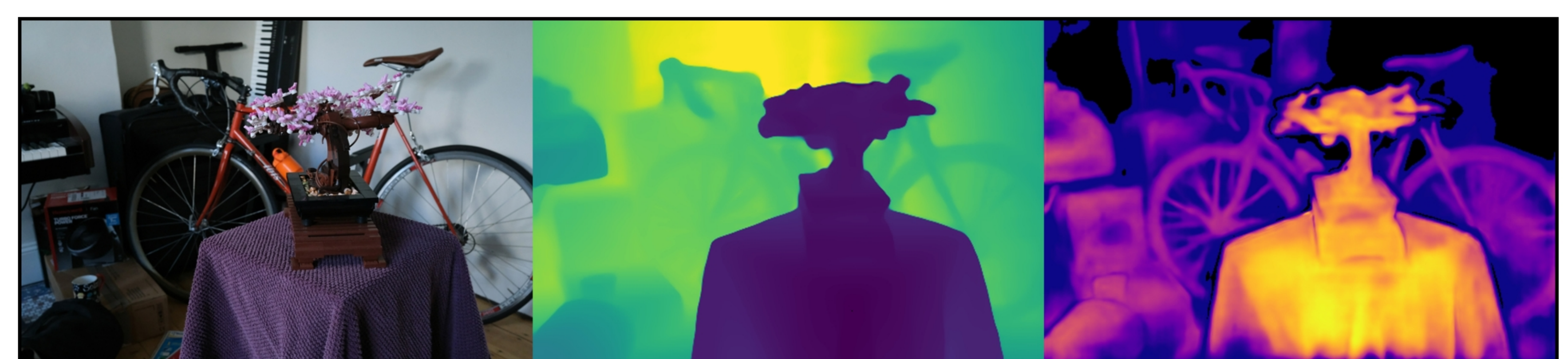
bonsai: VGGT | num_images=30 Original | Depth (max=2.25) | Confidence (max=4.34)
