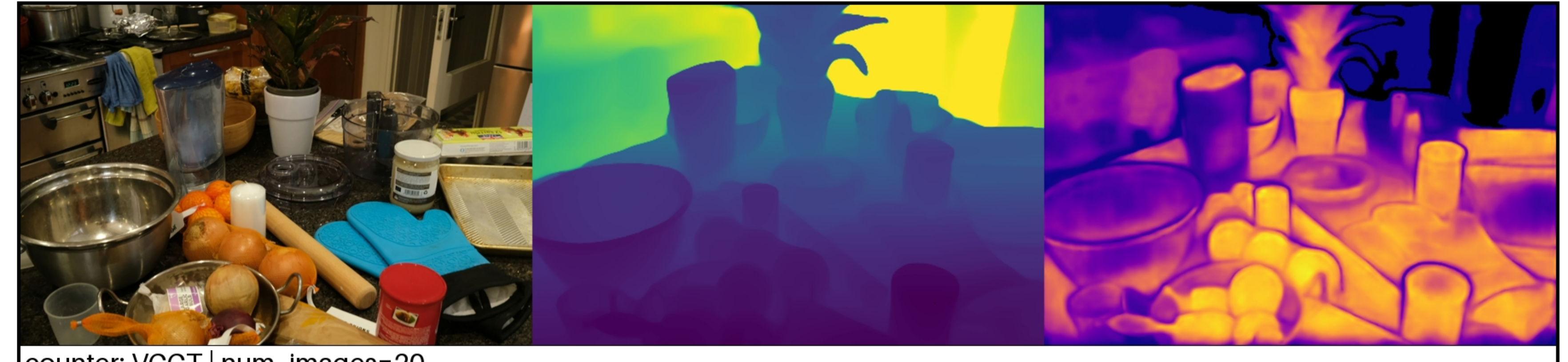
counter: VGGT | num_images=20 Original | Depth (max=2.90) | Confidence (max=12.59)
