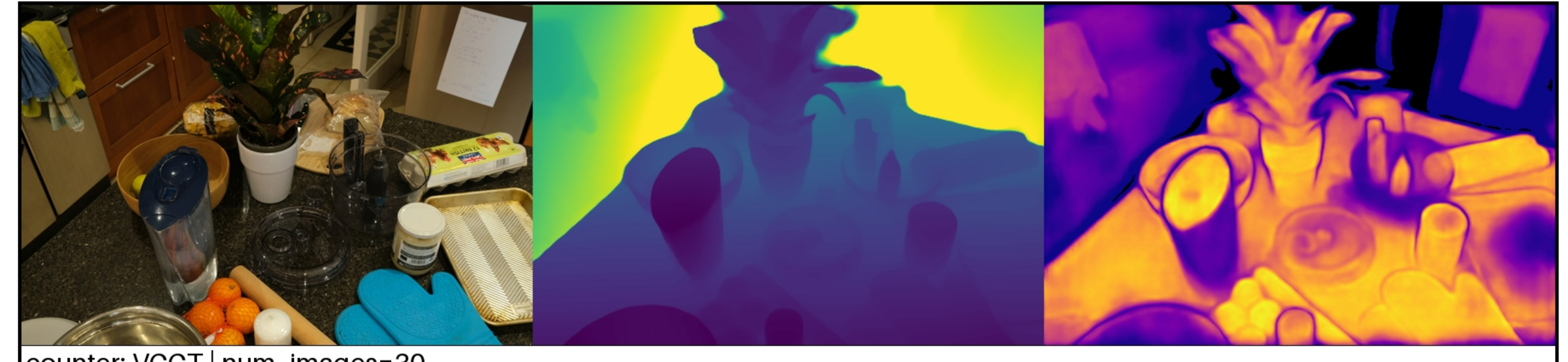
counter: VGGT | num_images=30 Original | Depth (max=2.48) | Confidence (max=13.28)
