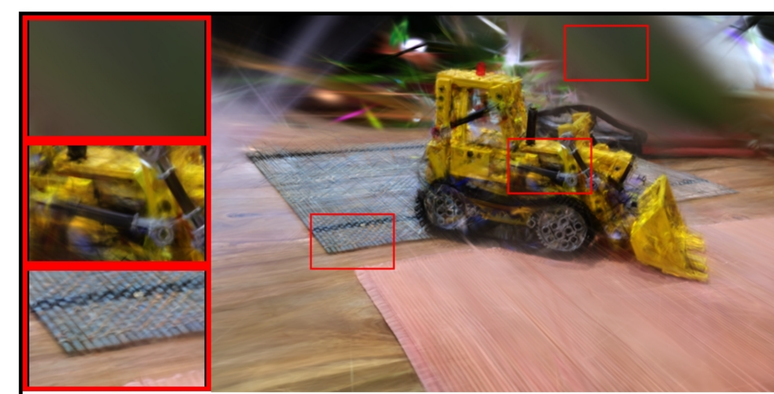
kitchen: COLMAP | num_images=20 PSNR: 16.58 | LPIPS: 0.4184 | SSIM: 0.3790
