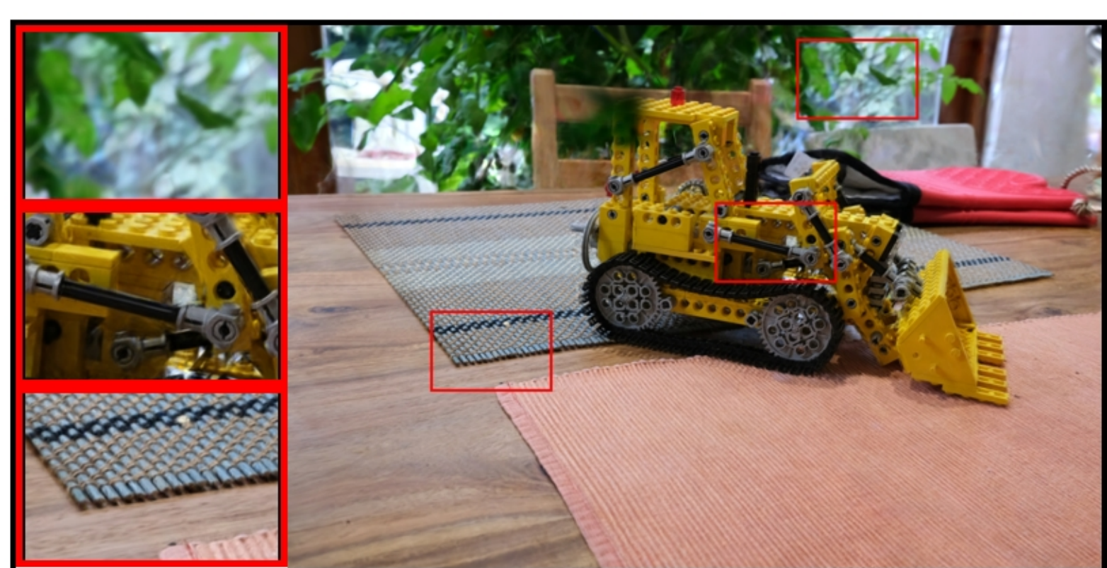
kitchen: VGGT | num_images=30 PSNR: 18.53 | LPIPS: 0.2711 | SSIM: 0.4427
