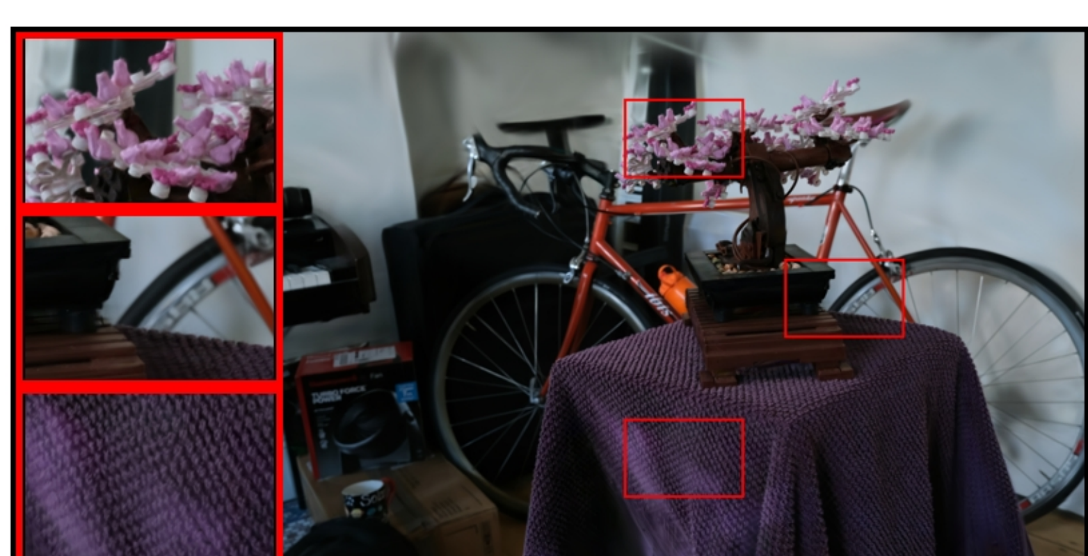
bonsai: COLMAP | num_images=100 PSNR: 27.83 | LPIPS: 0.1398 | SSIM: 0.8660
