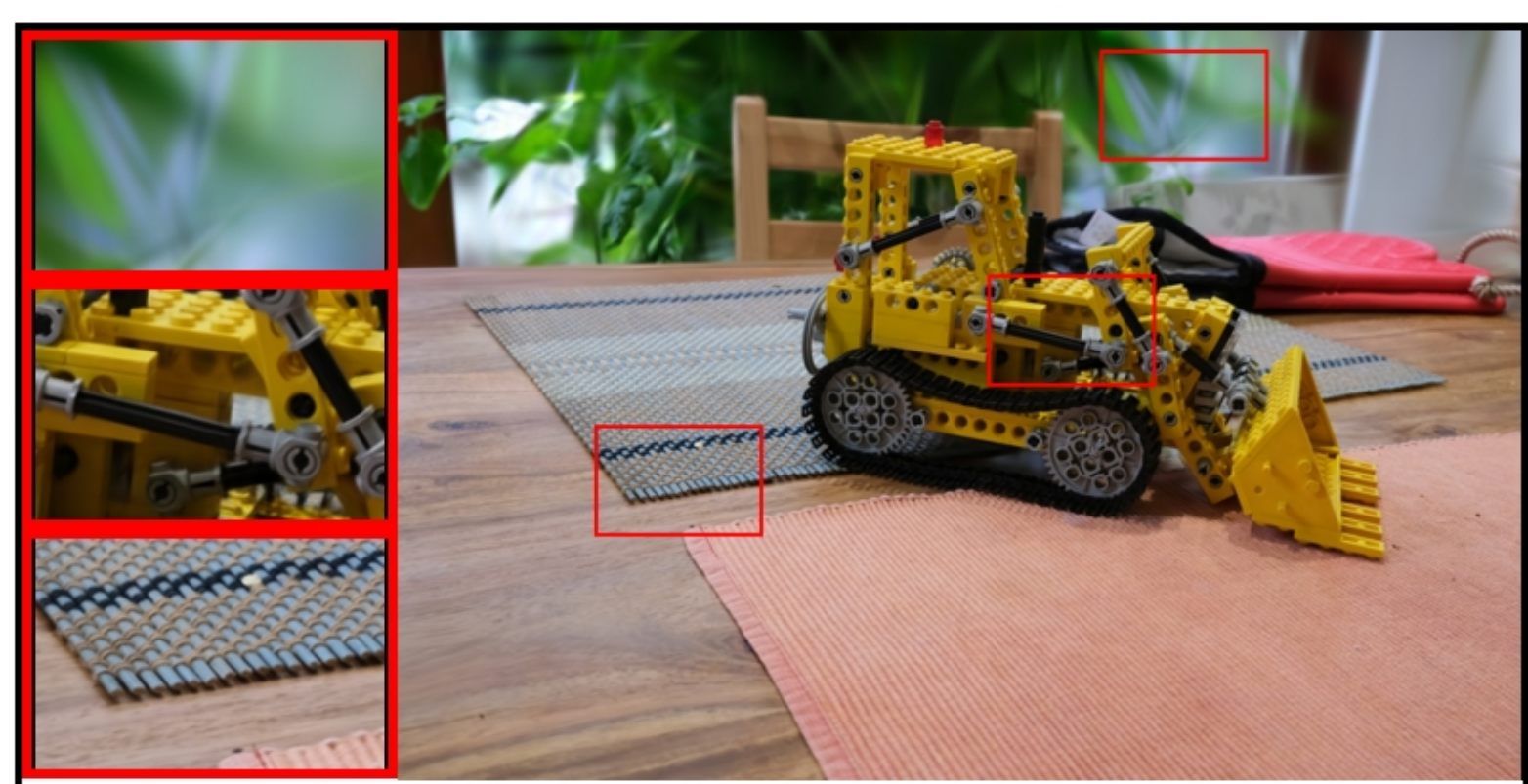
kitchen: COLMAP | num_images=100 PSNR: 21.72 | LPIPS: 0.1375 | SSIM: 0.4977
