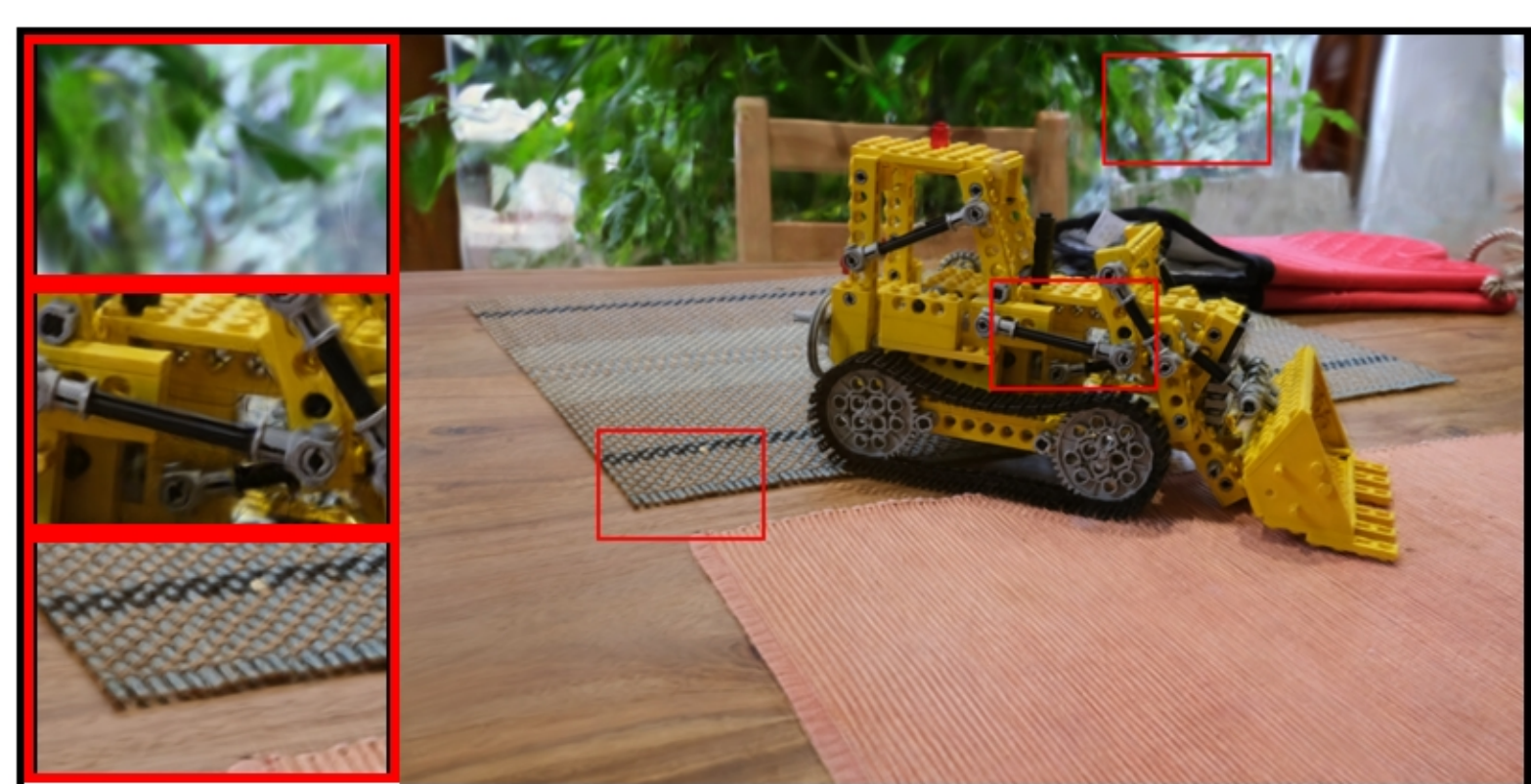
kitchen: VGGT | num_images=70 PSNR: 19.39 | LPIPS: 0.2471 | SSIM: 0.4489
