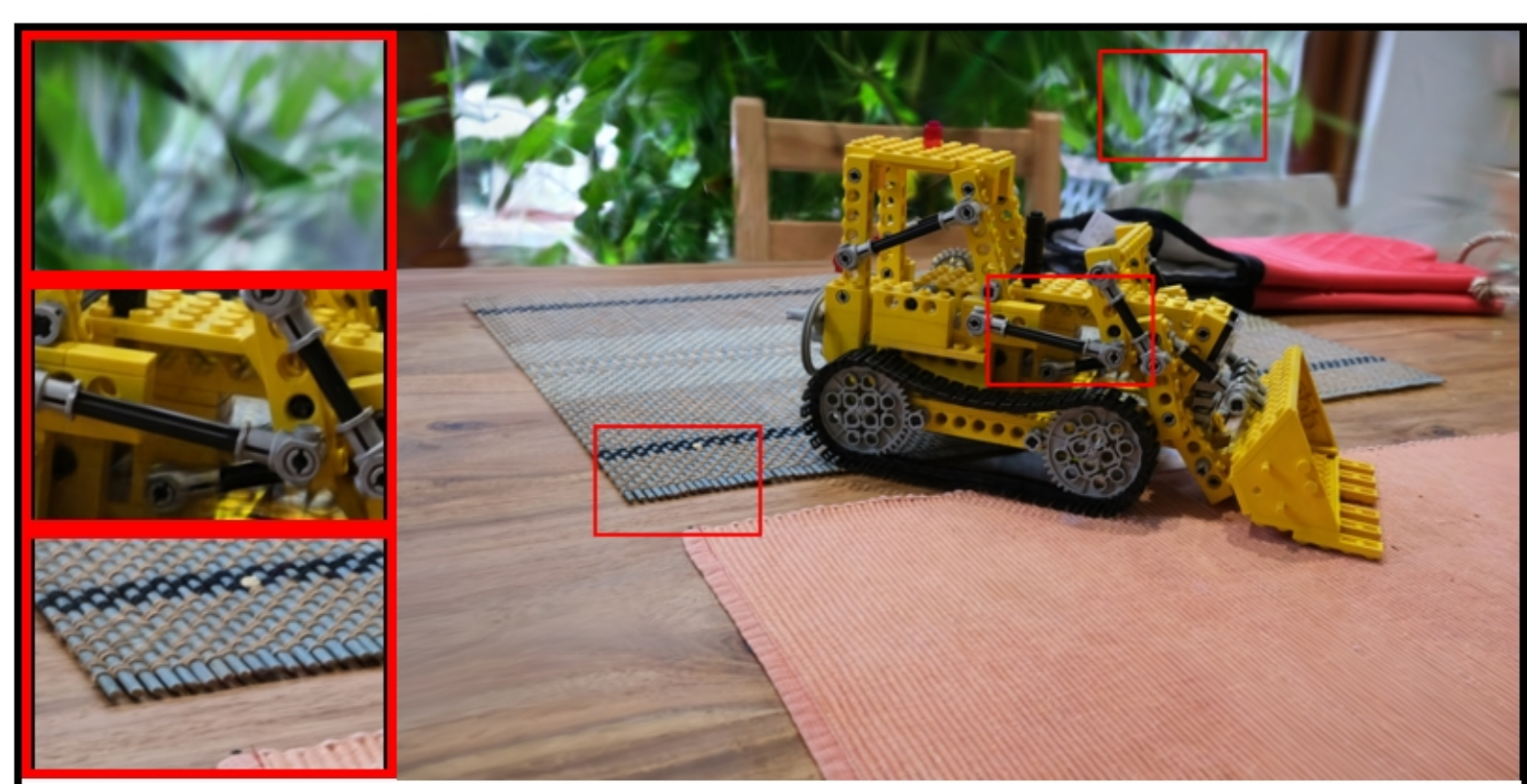
kitchen: COLMAP | num_images=30 PSNR: 20.04 | LPIPS: 0.2137 | SSIM: 0.4459
