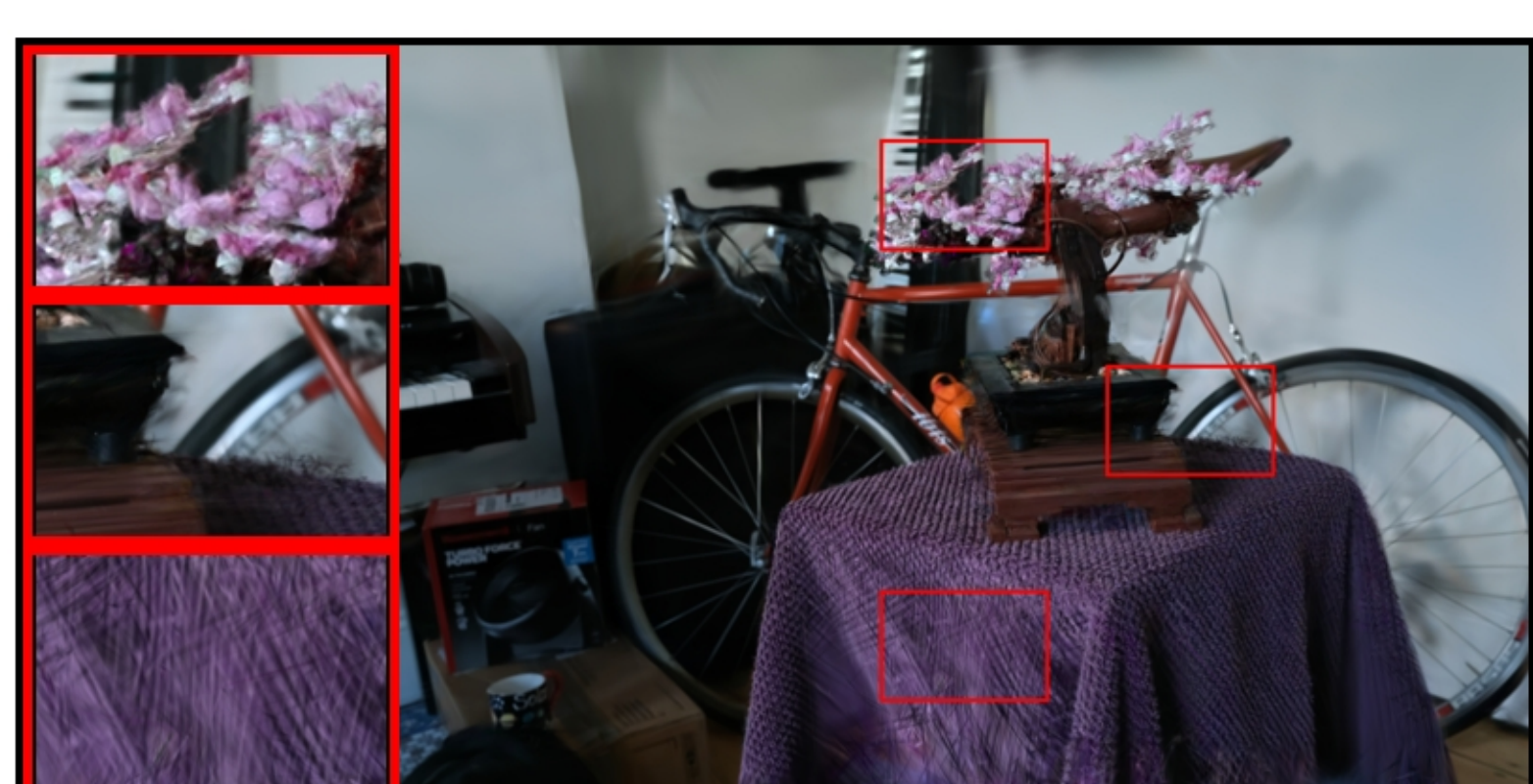
bonsai: COLMAP | num_images=40 PSNR: 20.85 | LPIPS: 0.2312 | SSIM: 0.6328
