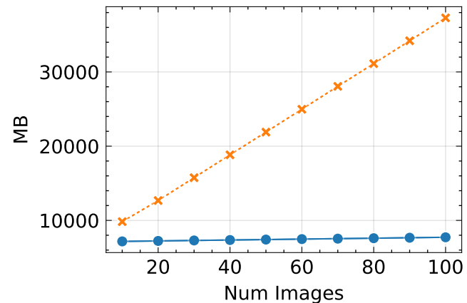
Peak Memory ↓ - counter
