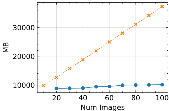
Peak Memory ↓ - kitchen
