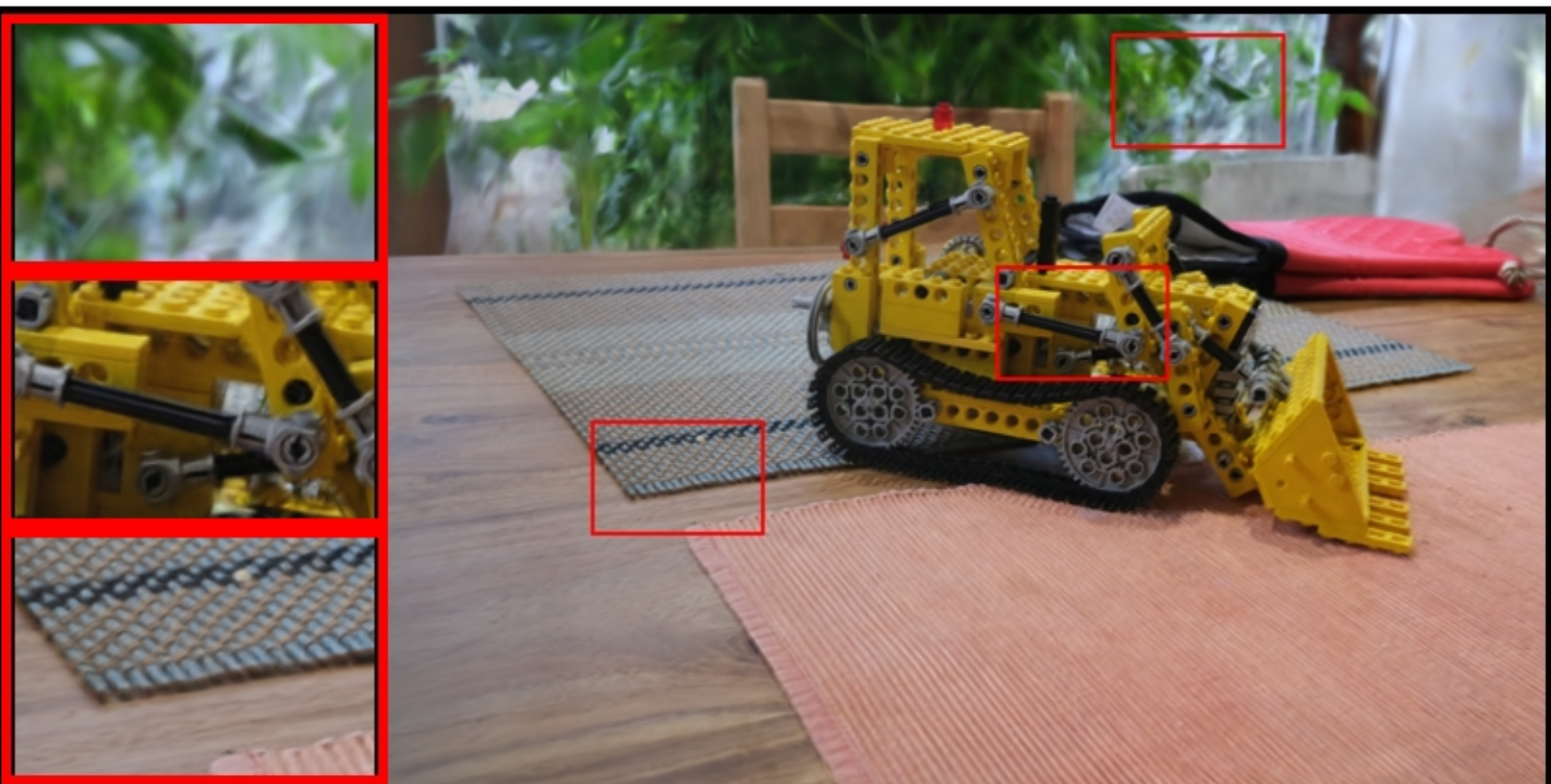
kitchen: VGGT | num_images=100 PSNR: 20.44 | LPIPS: 0.2303 | SSIM: 0.4850
