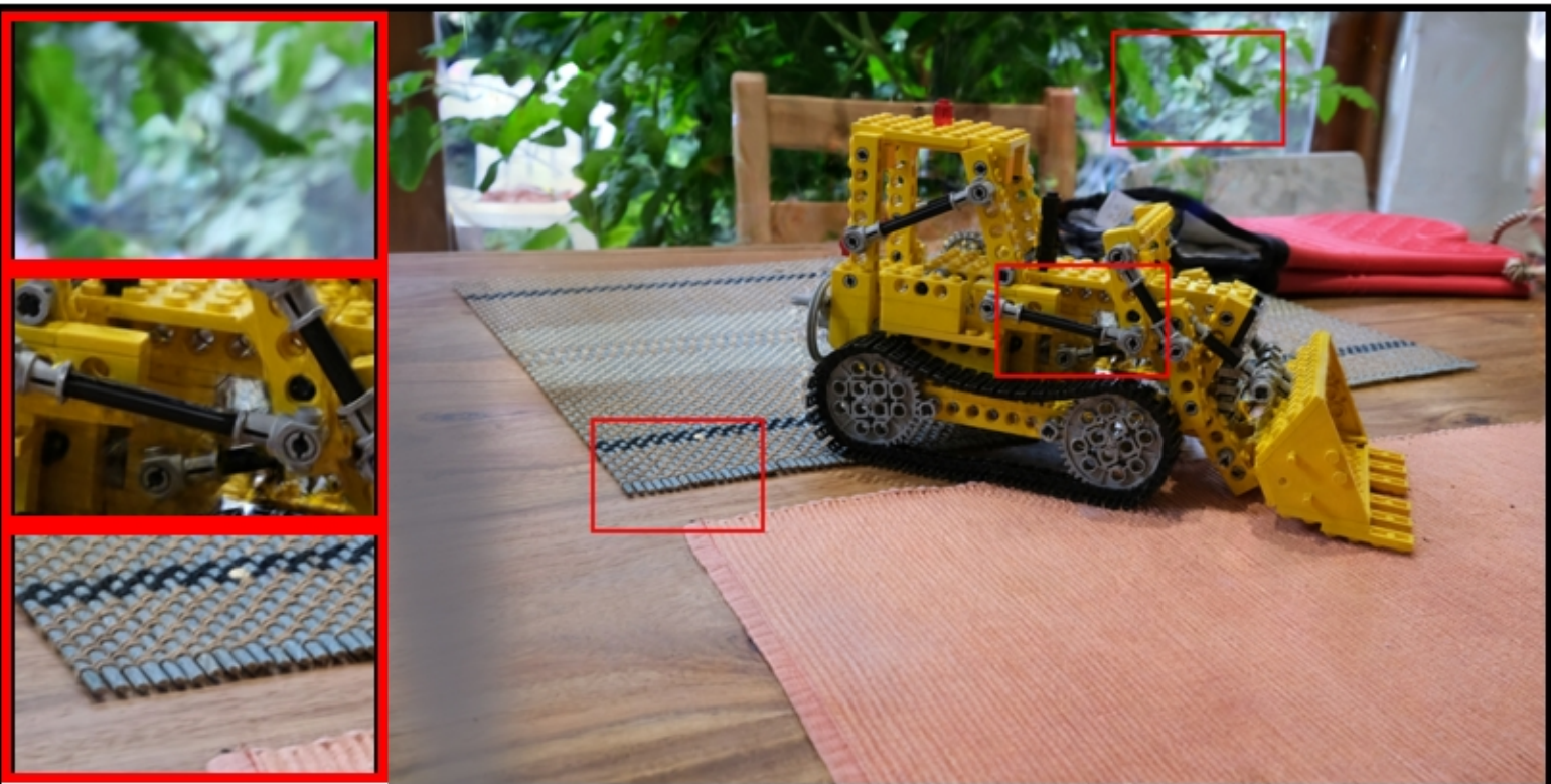
kitchen: VGGT | num_images=20 PSNR: 18.07 | LPIPS: 0.2931 | SSIM: 0.4224
