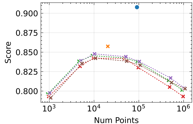
SSIM \uparrow
