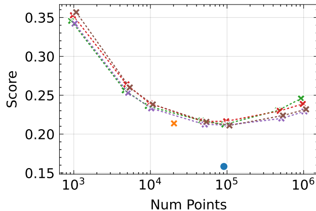
LPIPS \downarrow
