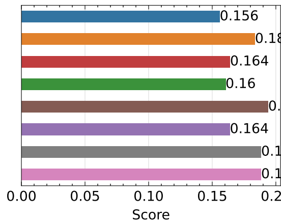
LPIPS ↓ - kitchen
