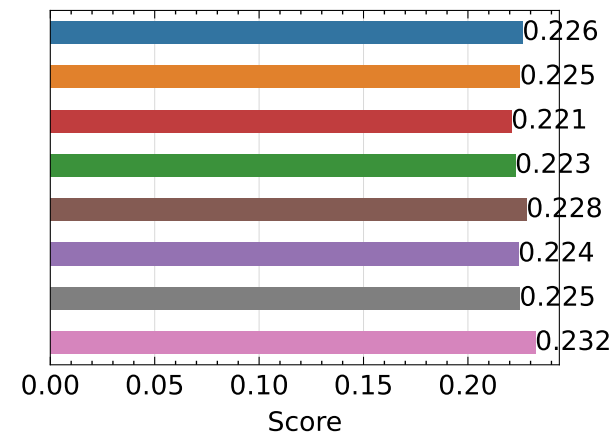
LPIPS ↓ - counter
