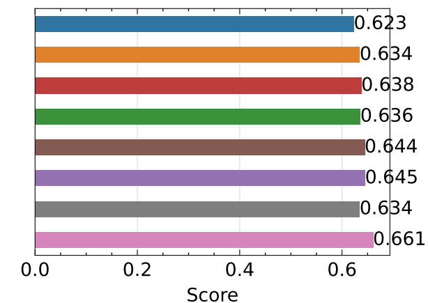
SSIM ↑ - counter
