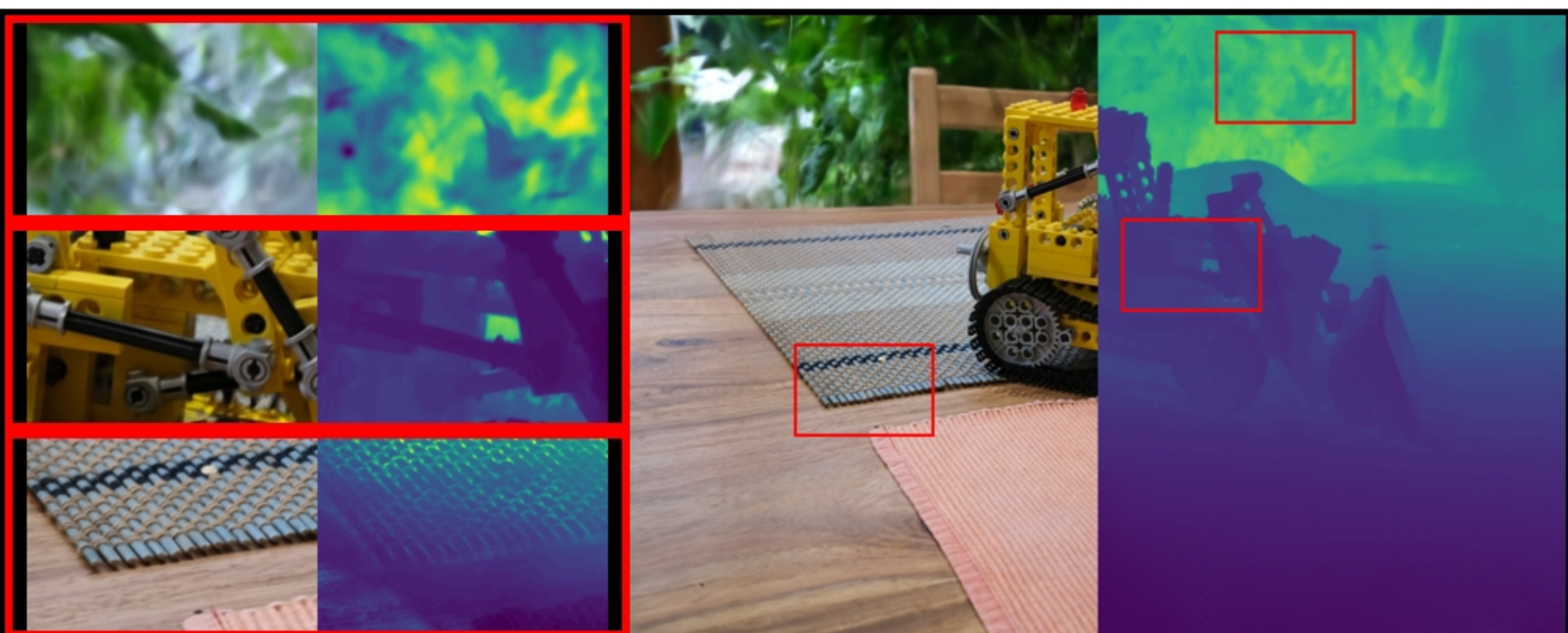
kitchen: VGGT | depth_lambda=0.0 PSNR: 21.23 | LPIPS: 0.1559 | SSIM: 0.5311
