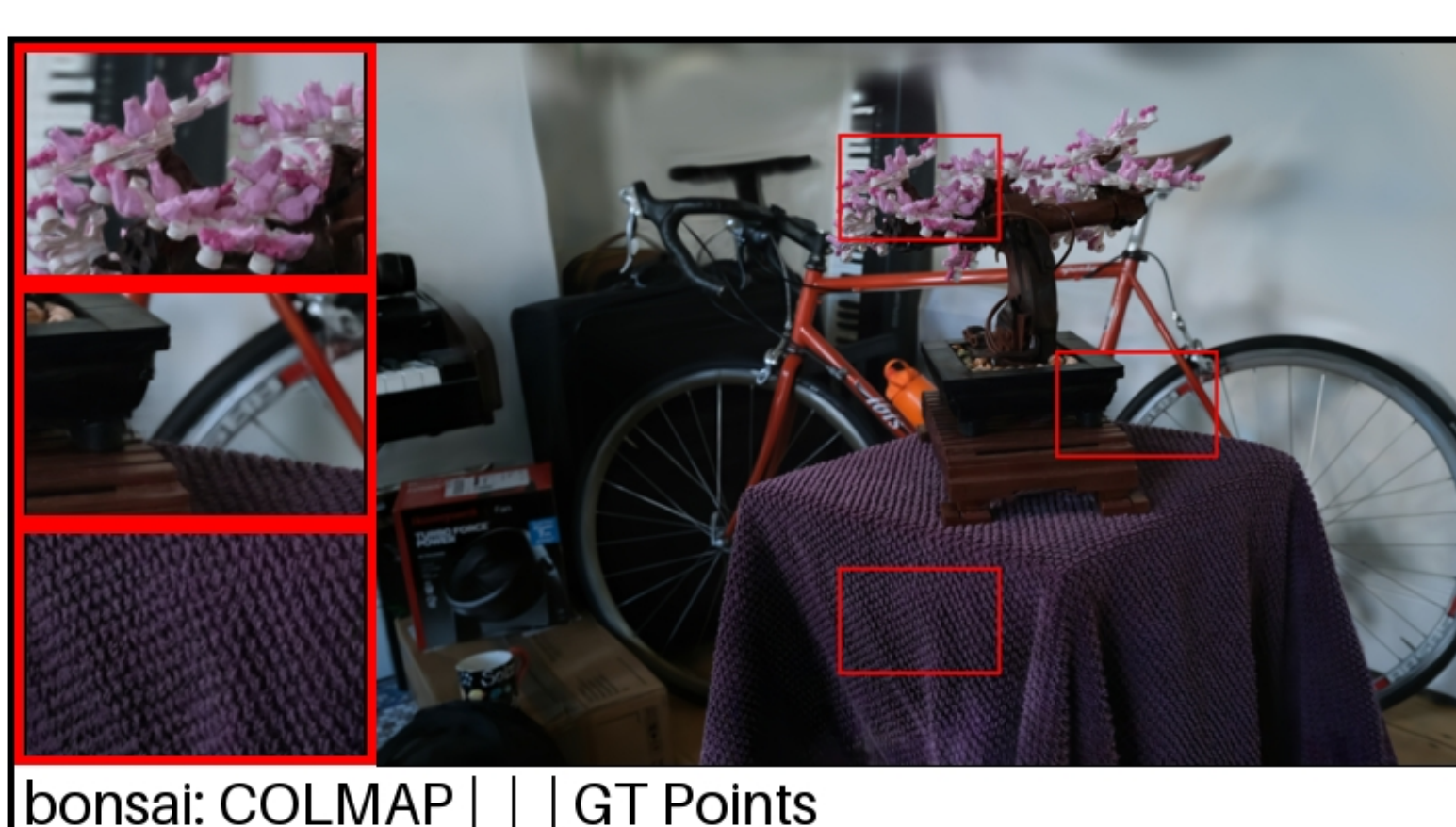
bonsai: COLMAP | | | GT Points PSNR: 27.99 | LPIPS: 0.1257 | SSIM: 0.8699
