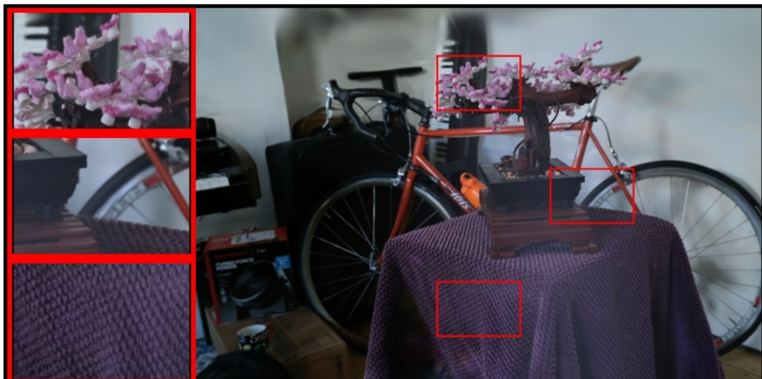
bonsai: COLMAP | GT Extrinsic | | GT Points PSNR: 31.55 | LPIPS: 0.1165 | SSIM: 0.9447
