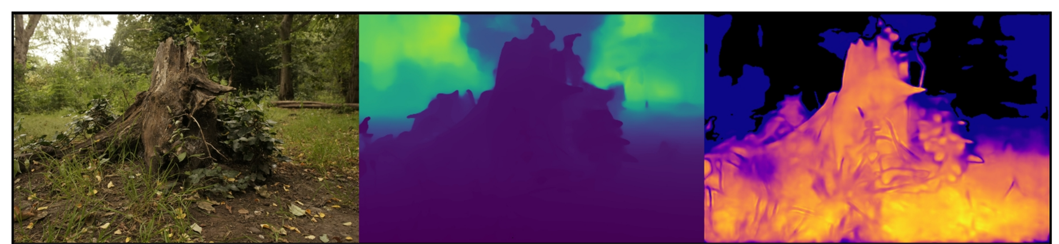
stump: VGGT | | GT Points Original | Depth (max=6.21) | Confidence (max=3.47)
