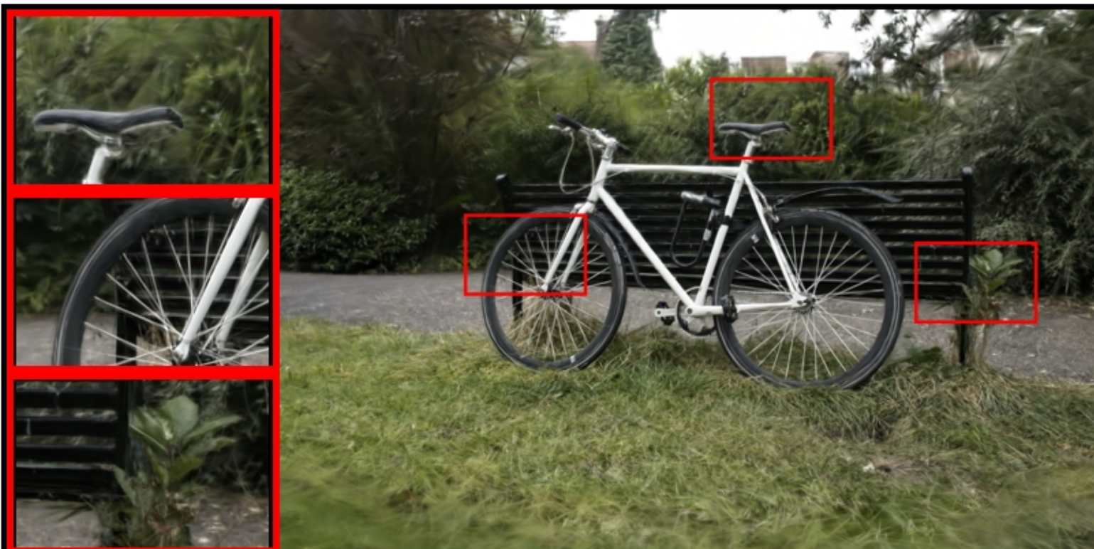
bicycle: VGGT | GT Extrinsic | | GT Points PSNR: 21.15 | LPIPS: 0.3393 | SSIM: 0.4684
