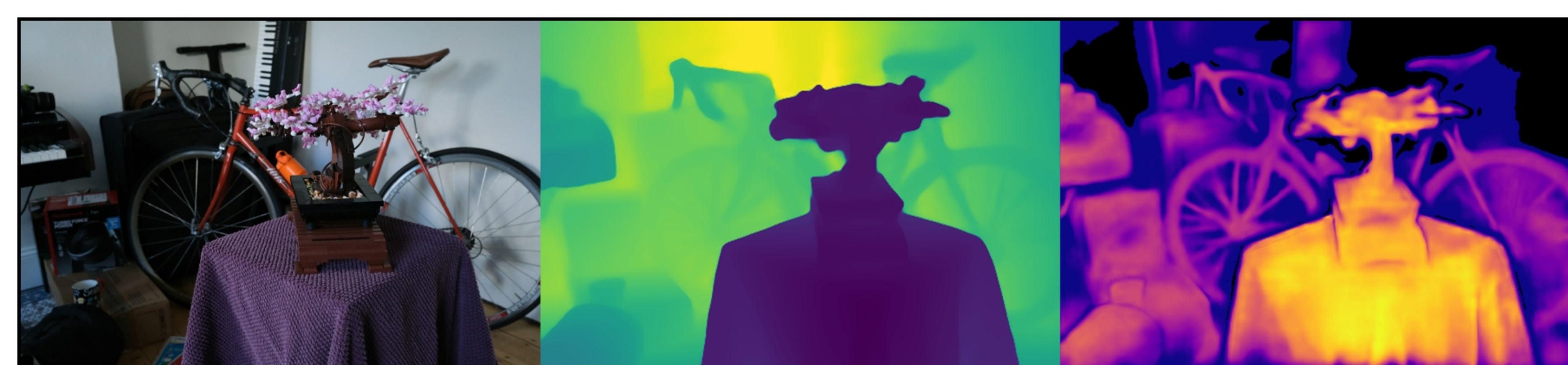
bonsai: VGGT | Random Init | Use BA Original | Depth (max=2.16) | Confidence (max=5.62)
