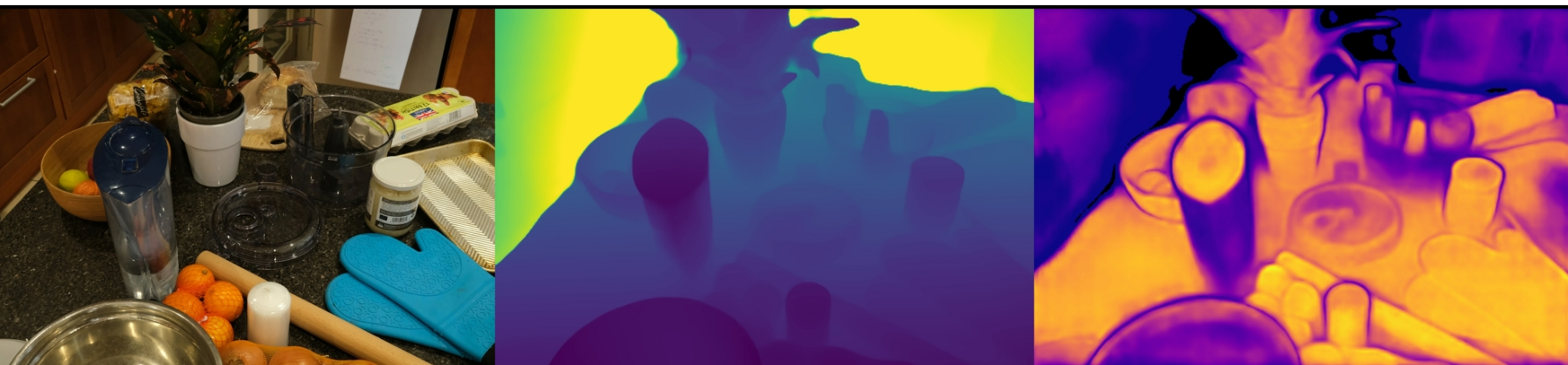
counter: VGGT | Random Init | Original | Depth (max=2.61) | Confidence (max=12.65)
