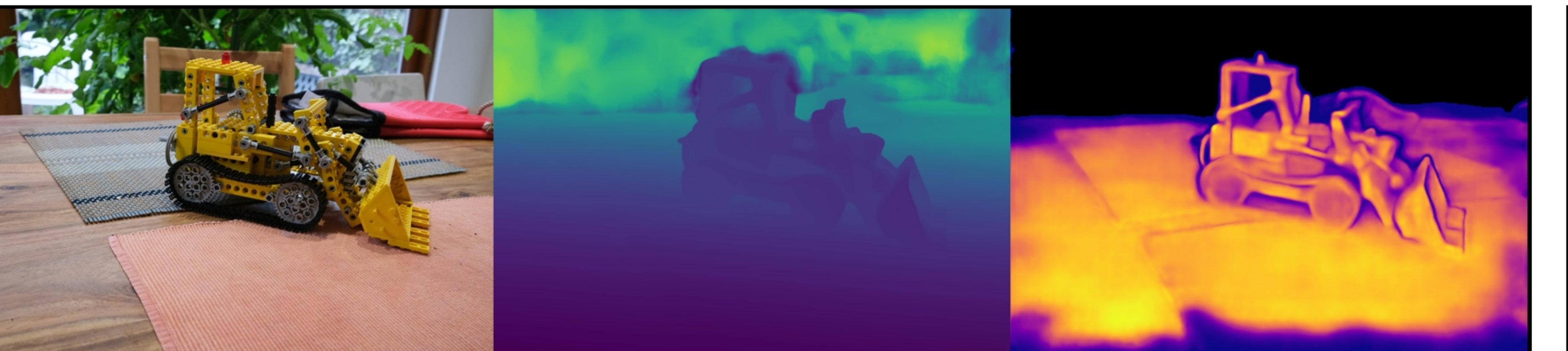
kitchen: VGGT | Random Init | Original | Depth (max=2.36) | Confidence (max=33.30)
