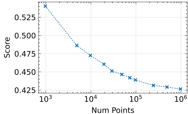
LPIPS \downarrow
