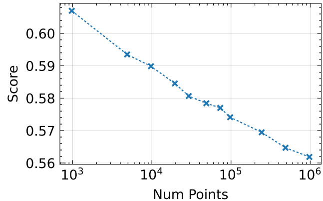
SSIM \uparrow
