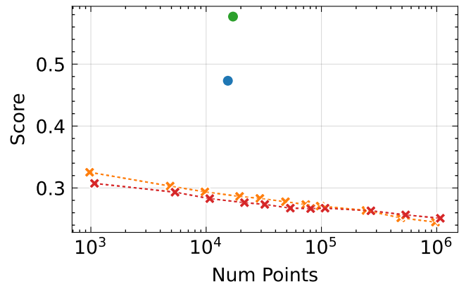
SSIM \uparrow
