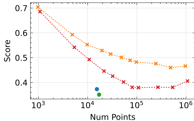
LPIPS \downarrow
