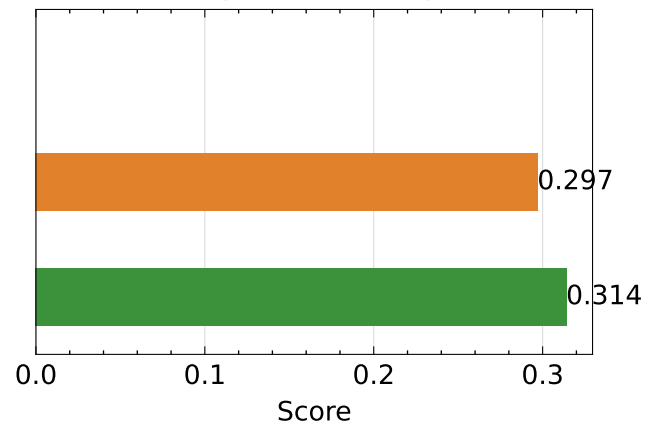
Composite Quality ↑
