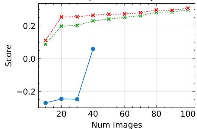
Composite Quality ↑
