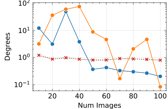
RRE ↓
