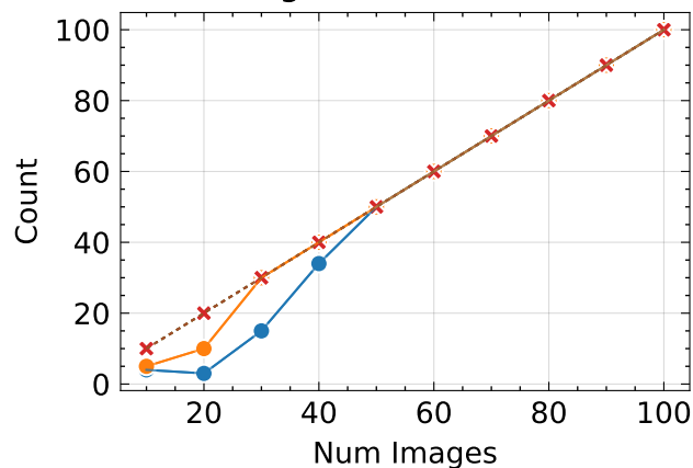
Aligned Cameras ↑
