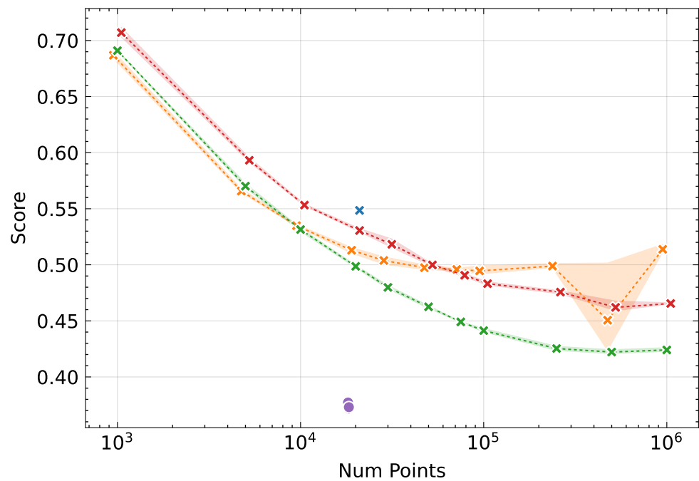
LPIPS \downarrow
