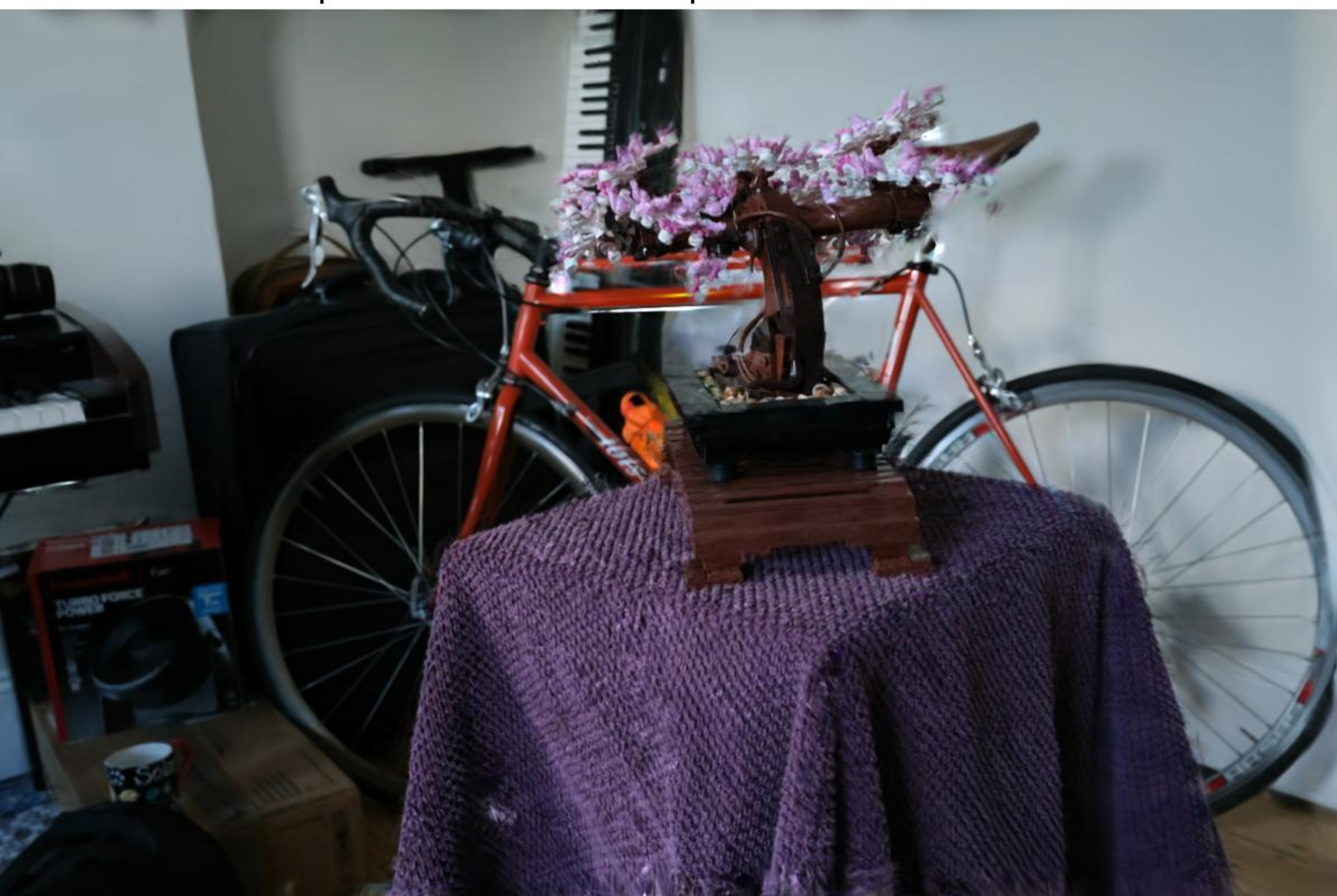
Config: VGGT | num_images=20 PSNR: 17.29 | LPIPS: 0.3292 | SSIM: 0.5486
