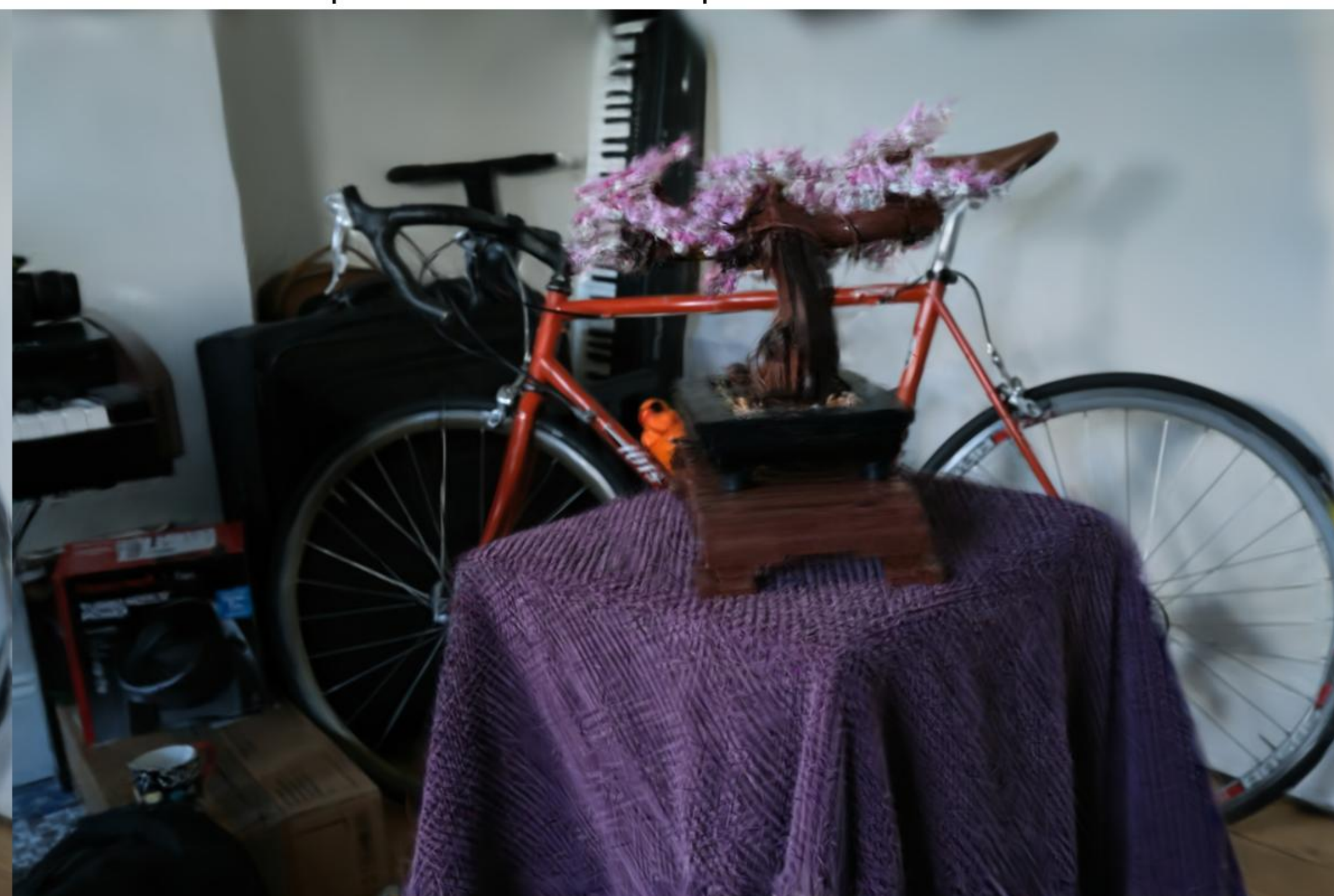
Config: VGGT | voxels | num_points=100000 PSNR: 17.97 | LPIPS: 0.3677 | SSIM: 0.5806
