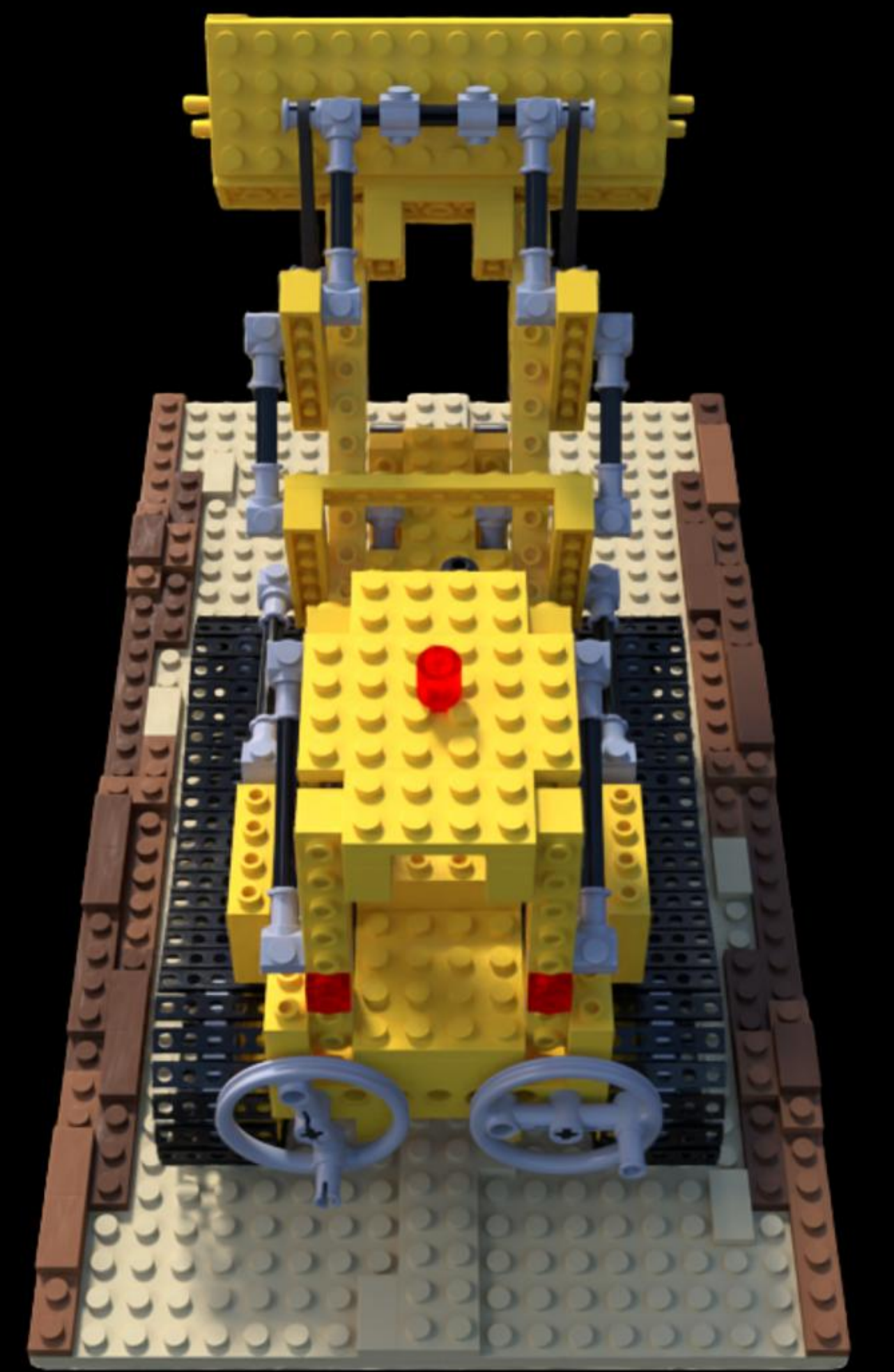
Config: VGGT | imagefps | num_points=87000 PSNR: 32.27 | LPIPS: 0.0313 | SSIM: 0.9822
