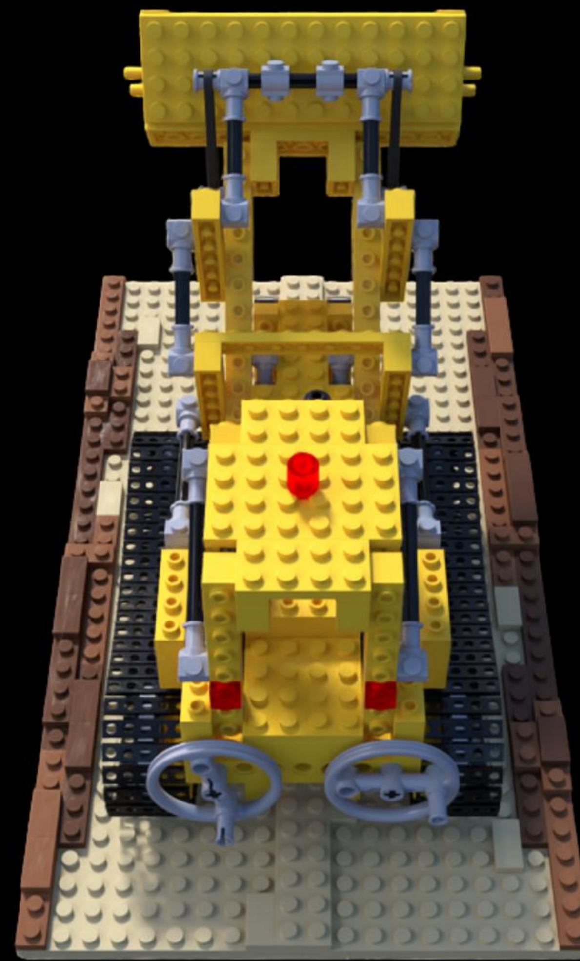
Config: VGGT | confidence | num_points=87000 PSNR: 32.64 | LPIPS: 0.0307 | SSIM: 0.9833
