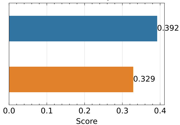
SSIM ↑ - bicycle
