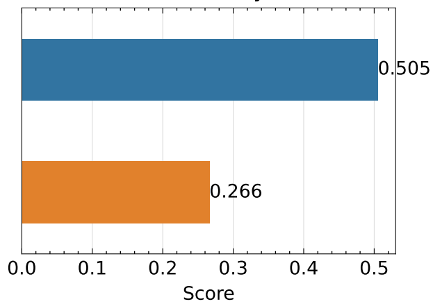
SSIM ↑ - bicycle
