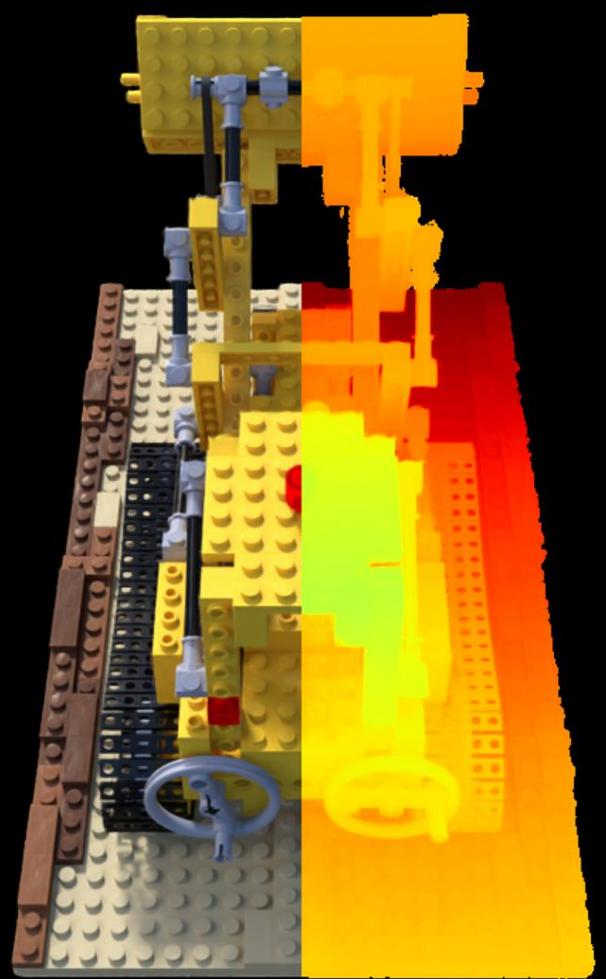
Config: VGGT | PSNR: 27.27 | LPIPS: 0.0467 | SSIM: 0.9379
