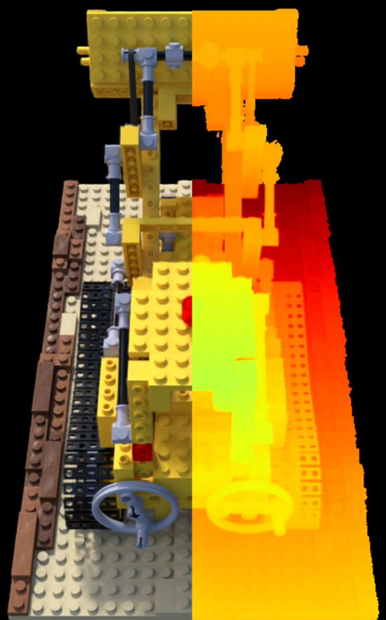
Config: VGGT | sigmoid PSNR: 27.35 | LPIPS: 0.0464 | SSIM: 0.9390
