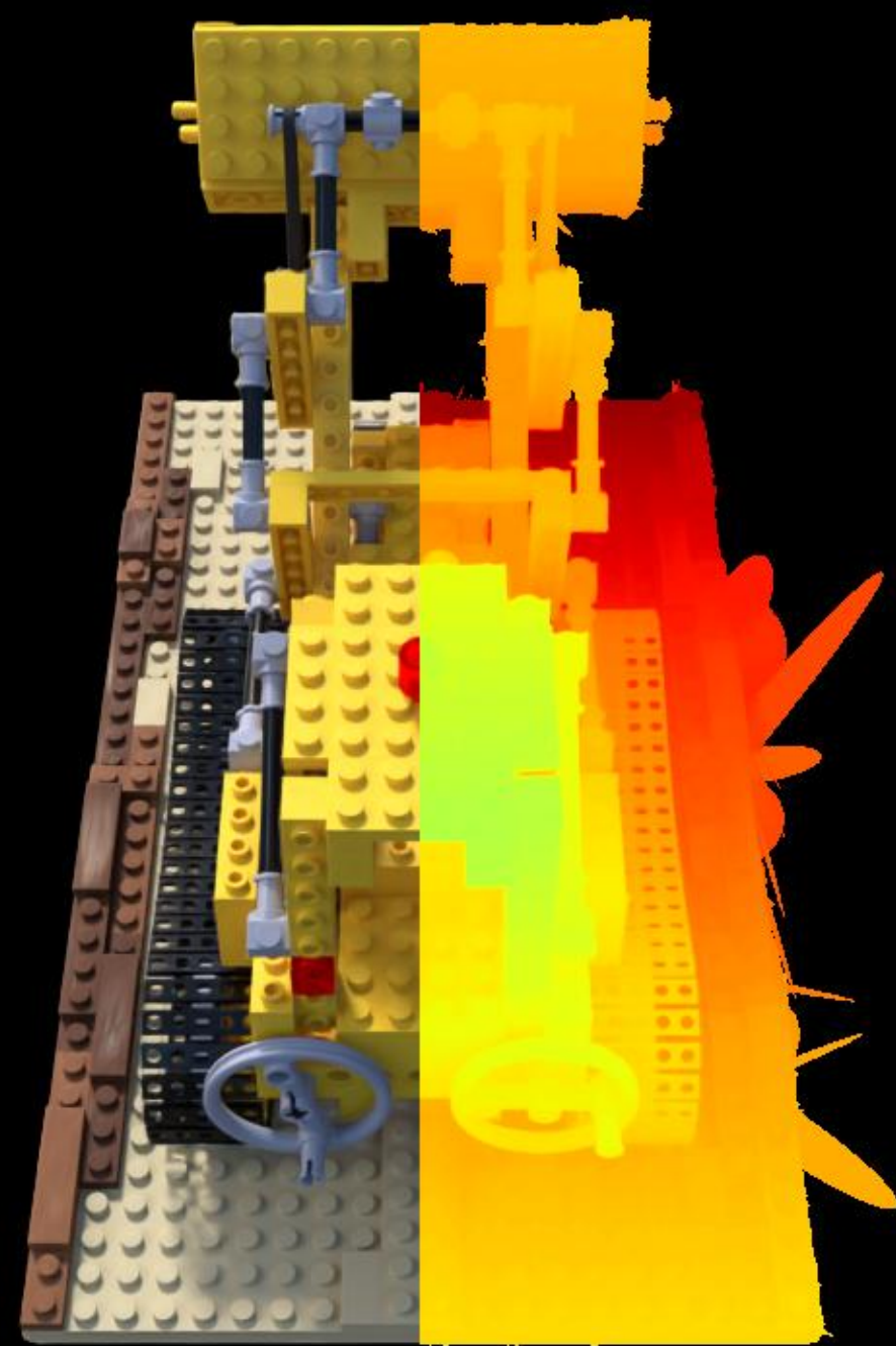
Config: COLMAP | | depth_lambda=0.0 PSNR: 25.22 | LPIPS: 0.0518 | SSIM: 0.9104
