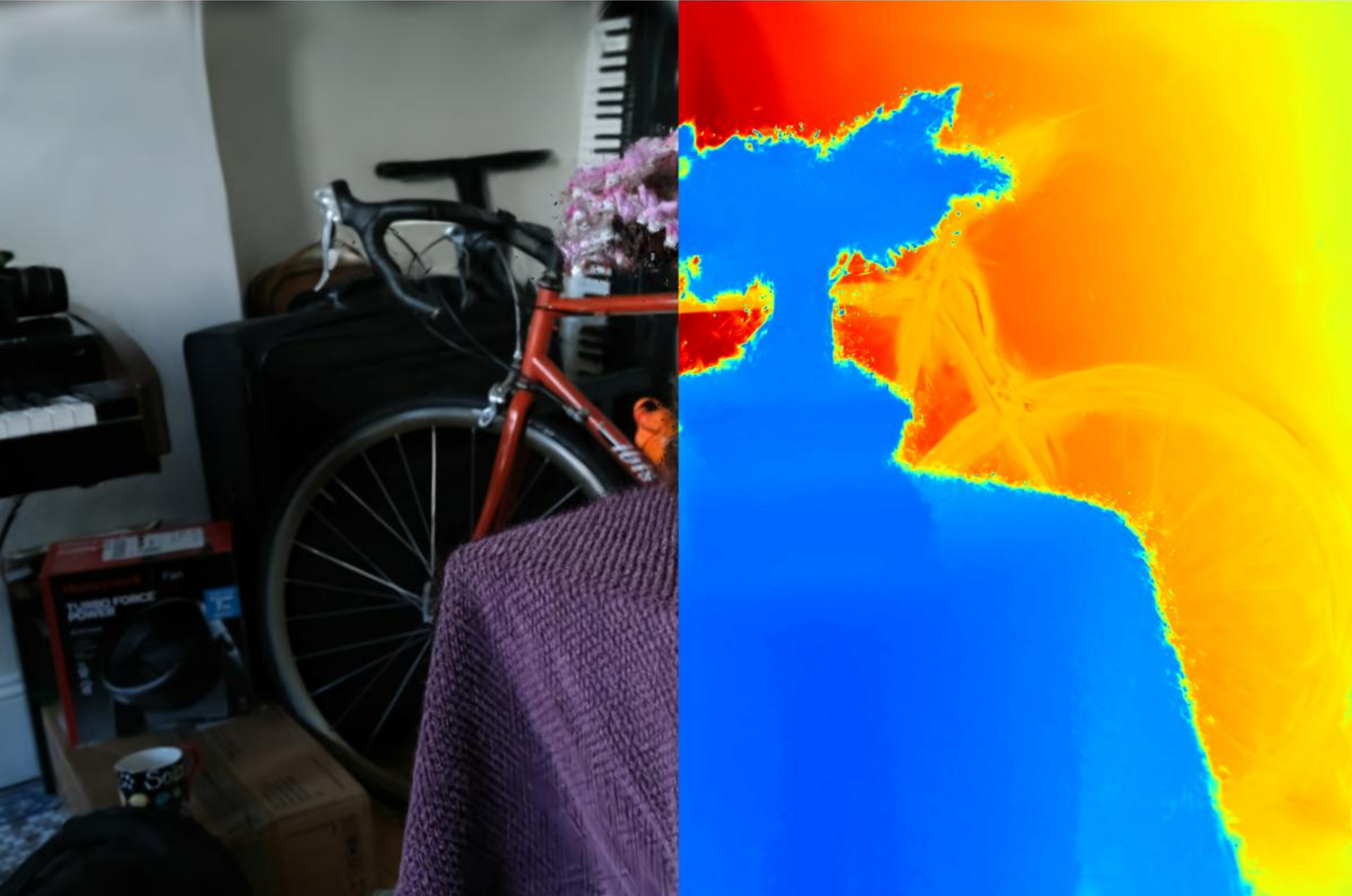
Config: VGGT | standard | points | depth_lambda=1.0 PSNR: 17.77 | LPIPS: 0.3277 | SSIM: 0.5660
