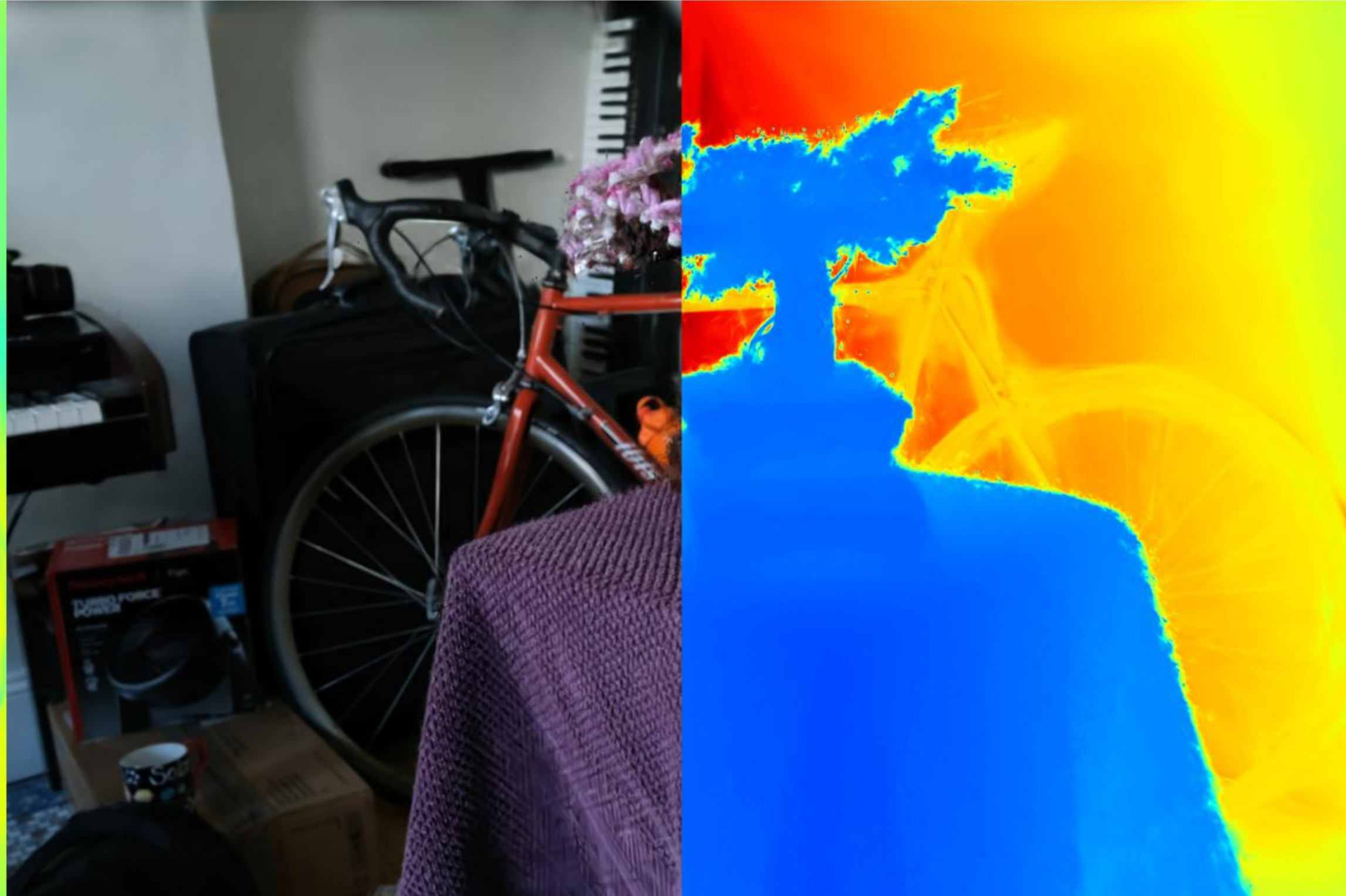
Config: VGGT | sigmoid | points | depth_lambda=1.0 PSNR: 17.51 | LPIPS: 0.3273 | SSIM: 0.5646
