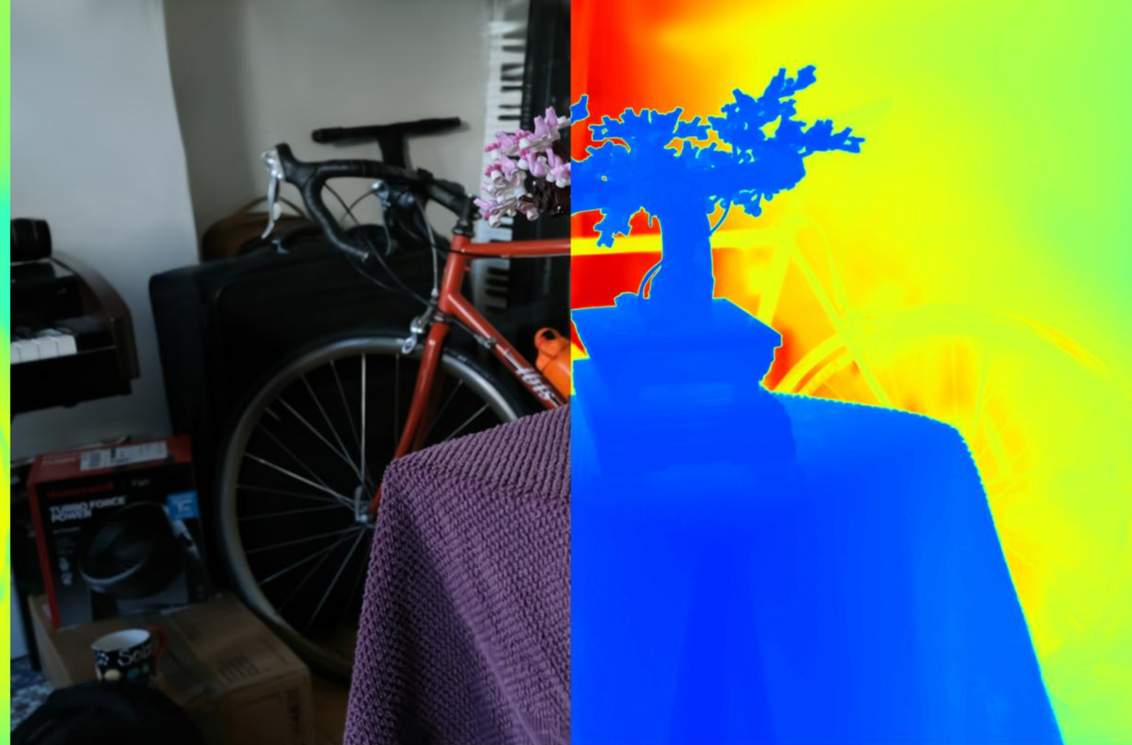
Config: COLMAP | | points | depth_lambda=0.01 PSNR: 30.56 | LPIPS: 0.1087 | SSIM: 0.9320
