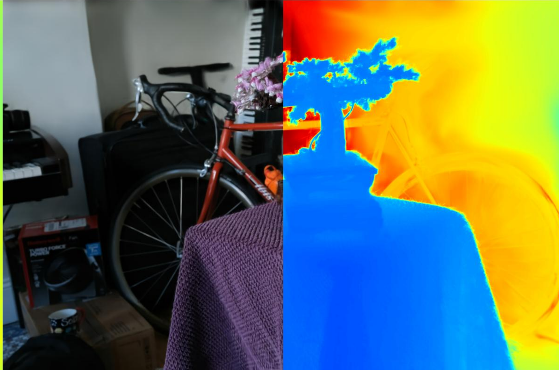
Config: VGGT | | points | depth_lambda=0.01 PSNR: 17.18 | LPIPS: 0.3282 | SSIM: 0.5660
