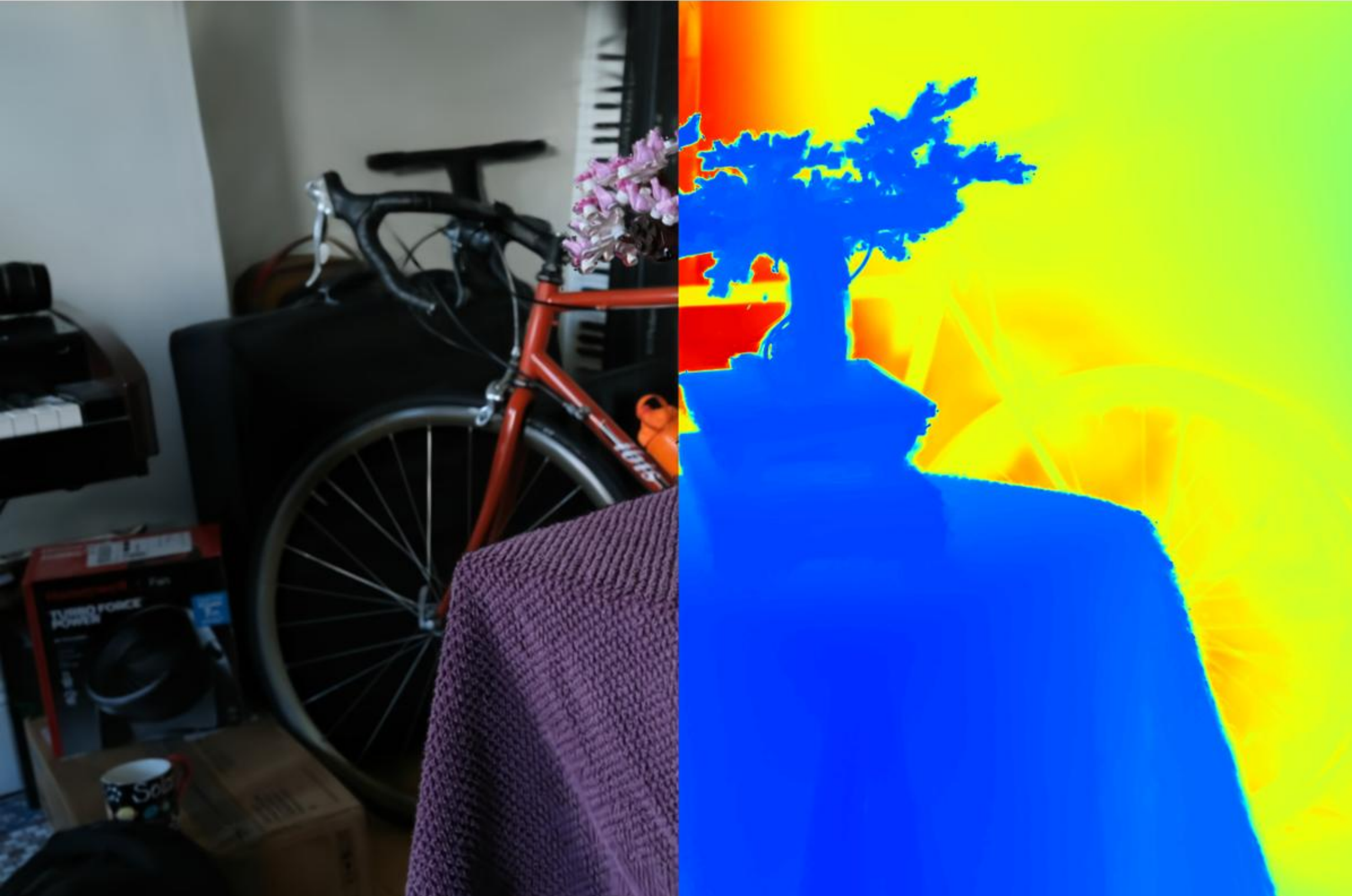
Config: COLMAP | | points | depth_lambda=1.0 PSNR: 23.65 | LPIPS: 0.1418 | SSIM: 0.7176
