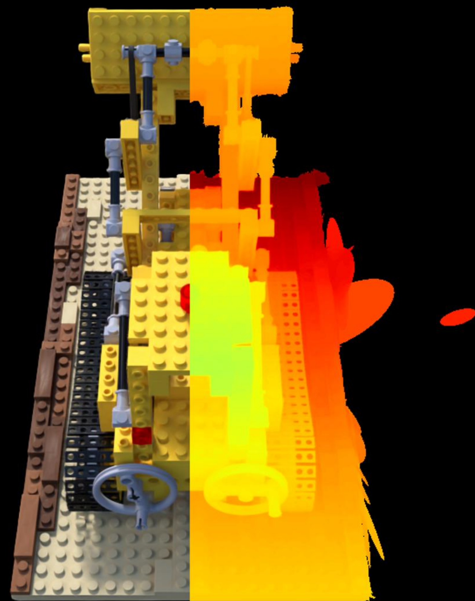
Config: COLMAP | | points | depth_lambda=0.01 PSNR: 25.12 | LPIPS: 0.0522 | SSIM: 0.9102
