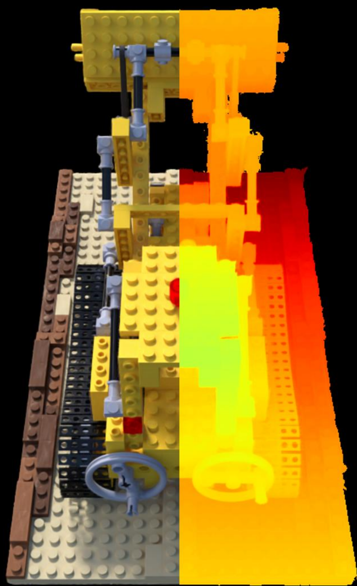
Config: VGGT | sigmoid | points | depth_lambda=0.01 PSNR: 25.82 | LPIPS: 0.0486 | SSIM: 0.9223
