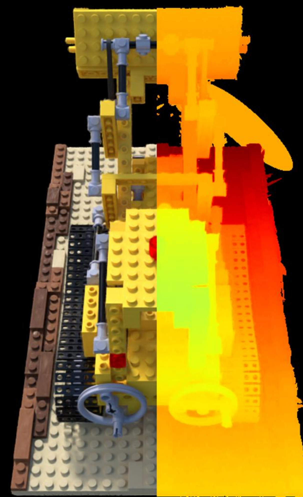
Config: VGGT | standard | points | depth_lambda=0.01 PSNR: 27.35 | LPIPS: 0.0429 | SSIM: 0.9460
