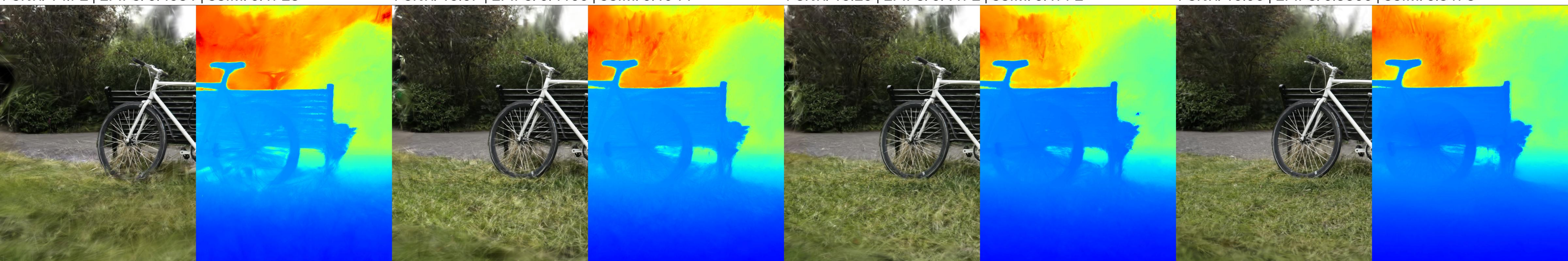
Config: VGGT | 1.0 | num_images=20 PSNR: 15.23 | LPIPS: 0.4718 | SSIM: 0.1905
