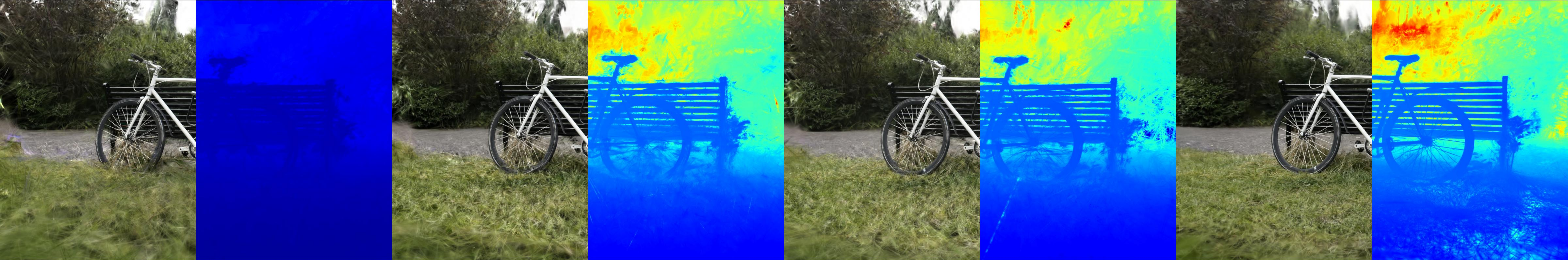
Config: VGGT | 0.0 | num_images=20 PSNR: 14.51 | LPIPS: 0.4855 | SSIM: 0.1769
