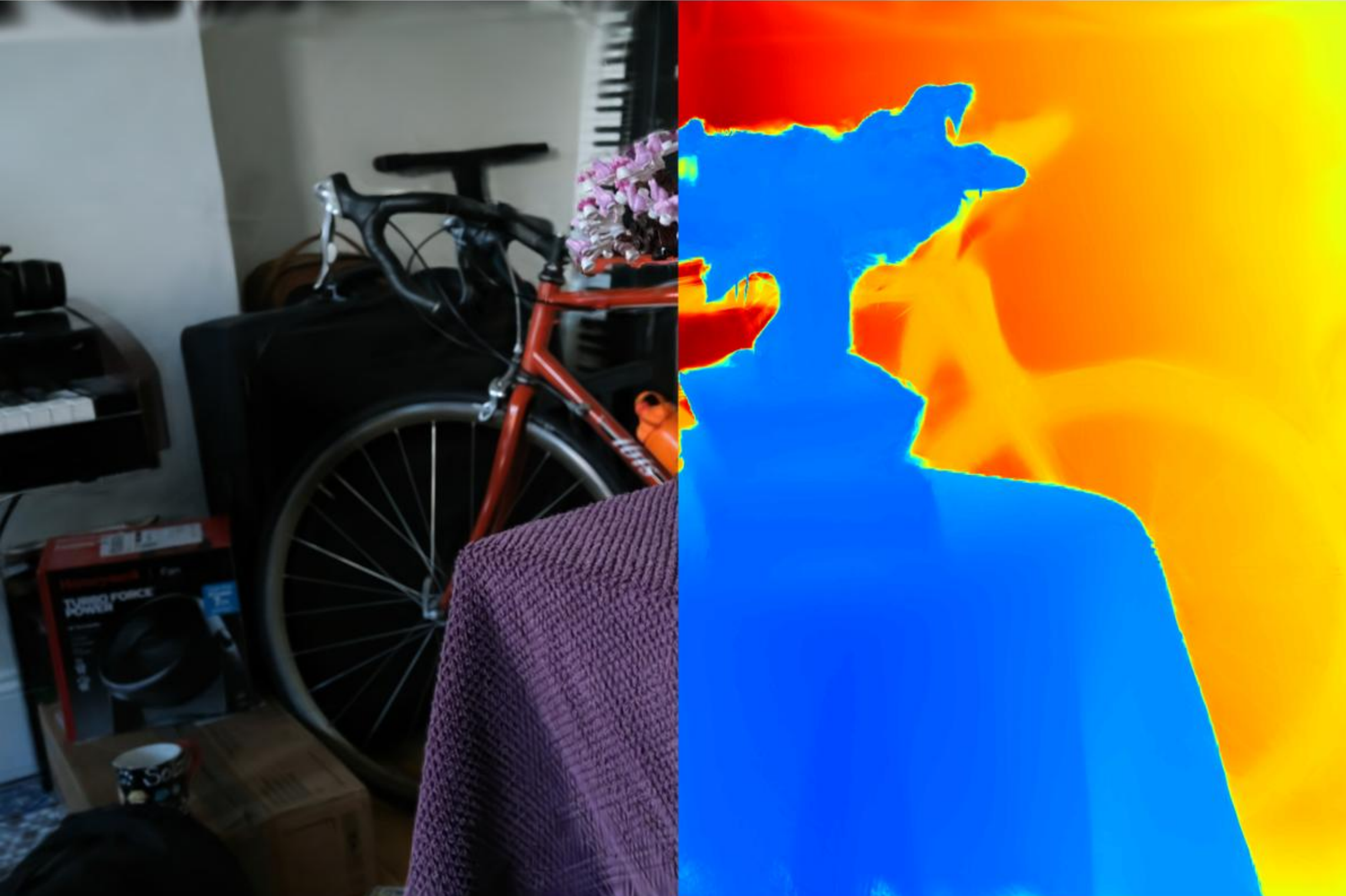
Config: VGGT | 1.0 | num_images=20 PSNR: 18.60 | LPIPS: 0.2804 | SSIM: 0.5724
