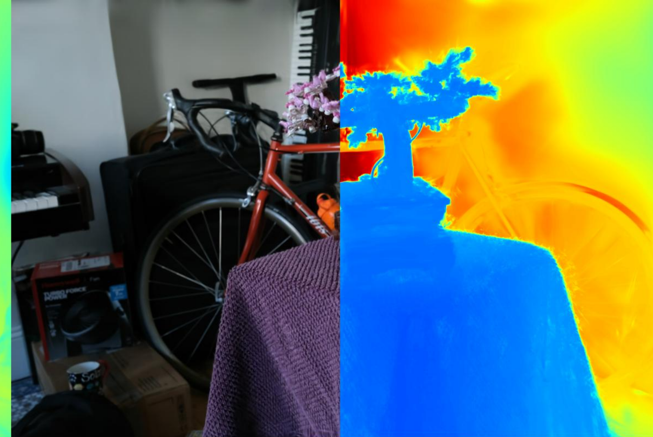
Config: VGGT | 0.0 | num_images=40 PSNR: 16.99 | LPIPS: 0.3291 | SSIM: 0.5622
