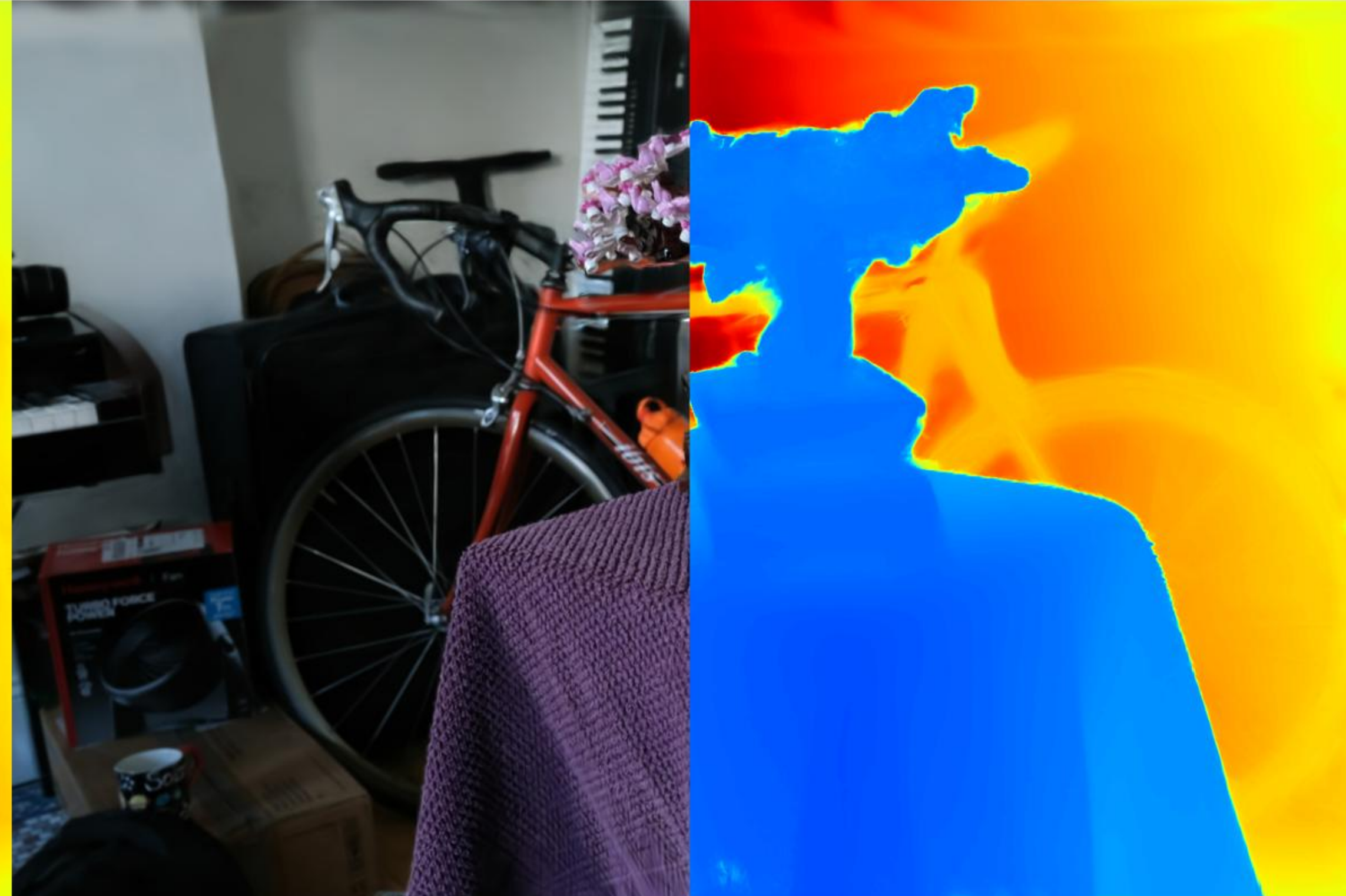
Config: VGGT | 1.0 | num_images=30 PSNR: 17.17 | LPIPS: 0.2980 | SSIM: 0.5673
