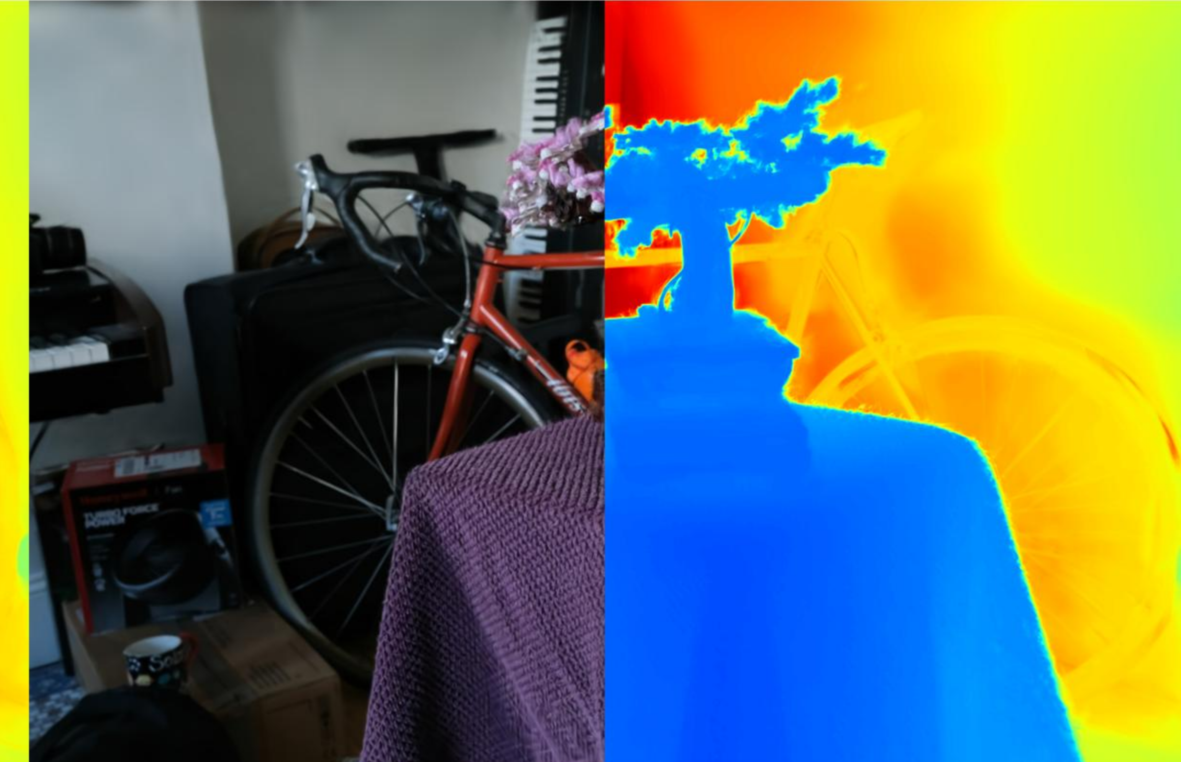
Config: VGGT | 0.01 | num_images=100 PSNR: 17.31 | LPIPS: 0.3237 | SSIM: 0.5654
