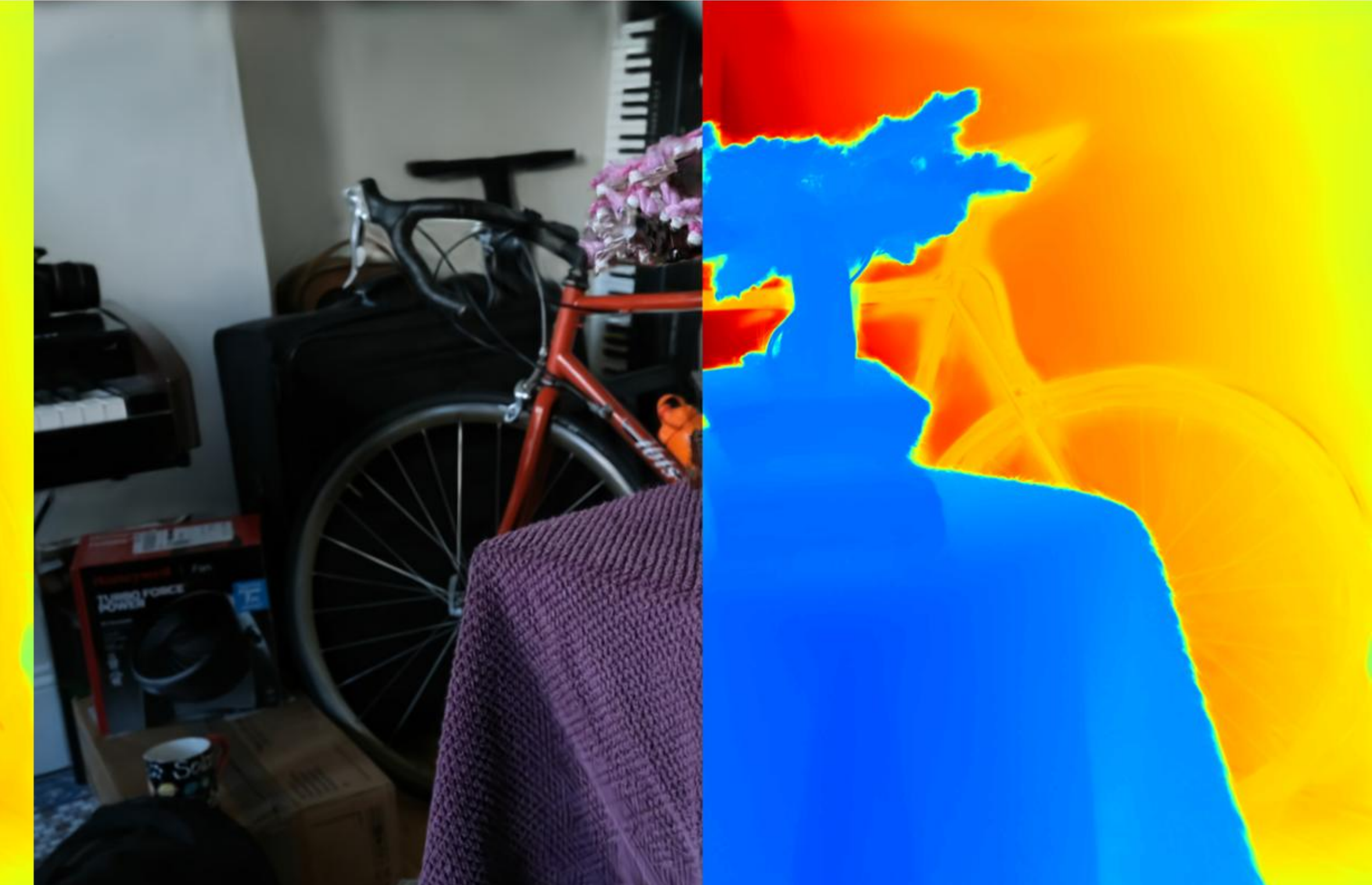
Config: VGGT | 0.1 | num_images=100 PSNR: 17.37 | LPIPS: 0.3271 | SSIM: 0.5631
