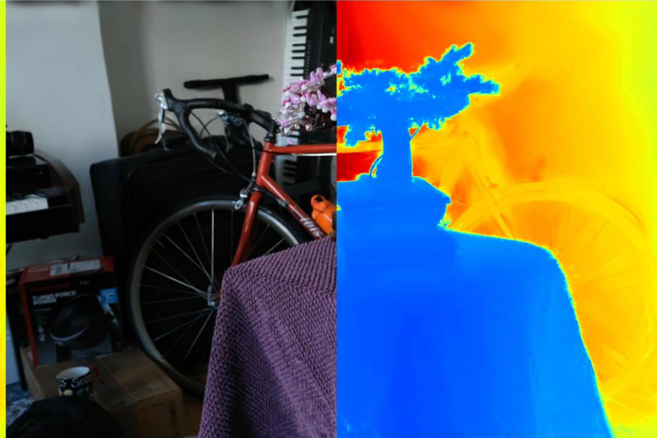
Config: VGGT | 0.01 | num_images=30 PSNR: 17.21 | LPIPS: 0.2916 | SSIM: 0.5648
