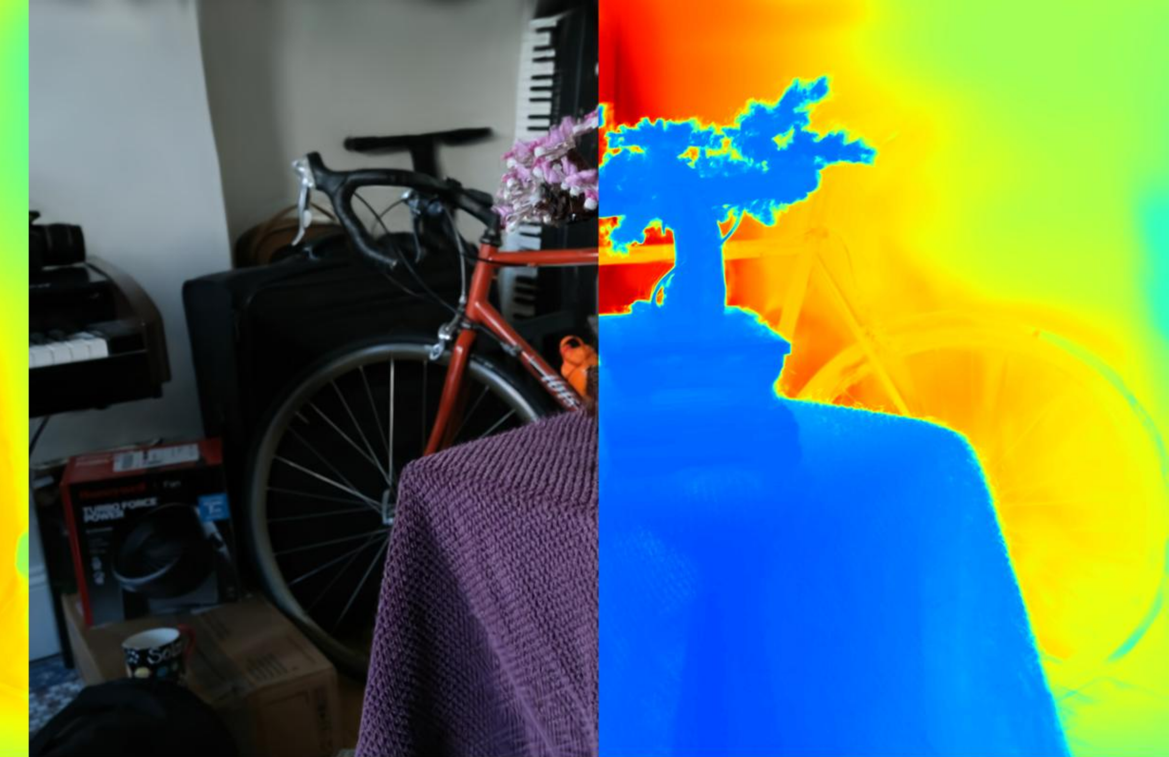
Config: VGGT | 0.0 | num_images=100 PSNR: 17.32 | LPIPS: 0.3256 | SSIM: 0.5684
