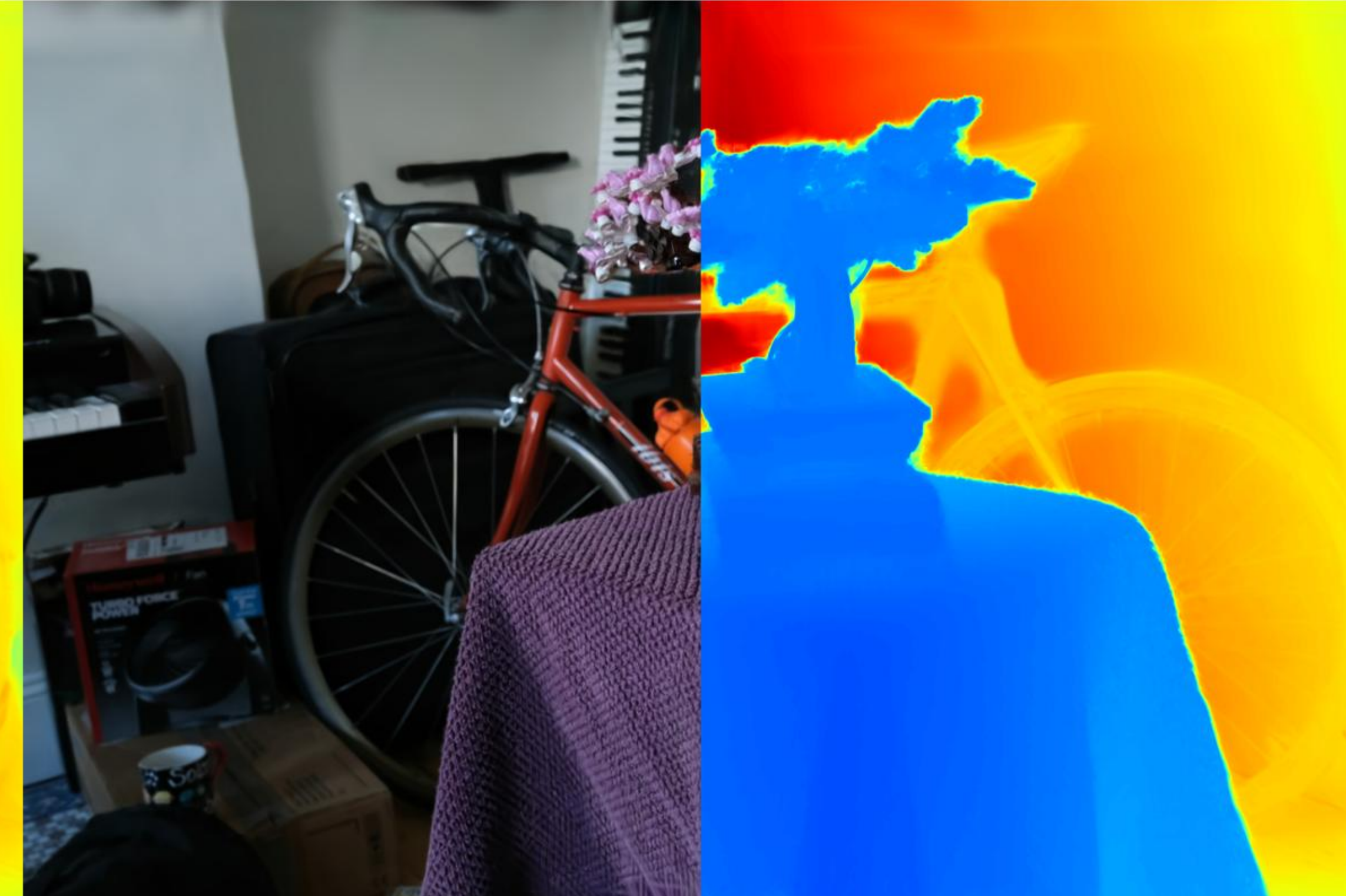
Config: VGGT | 0.1 | num_images=40 PSNR: 17.11 | LPIPS: 0.3296 | SSIM: 0.5640
