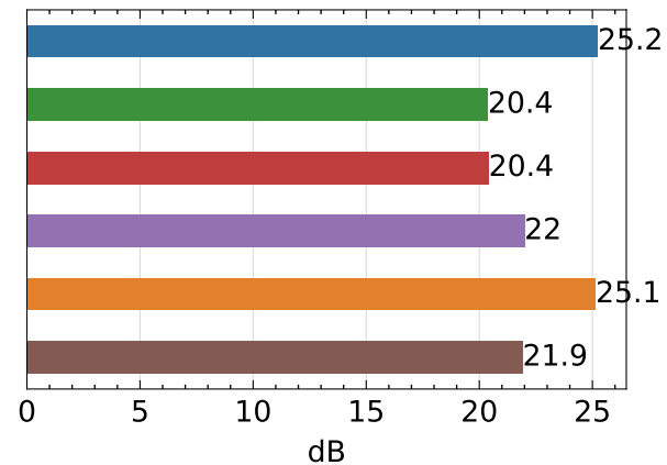
Composite Quality ↑
