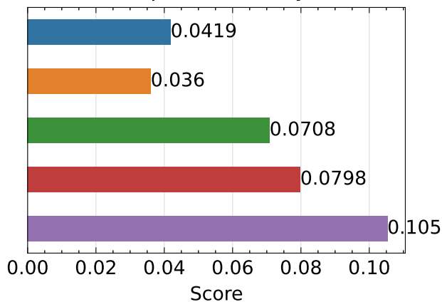
Composite Quality ↑
