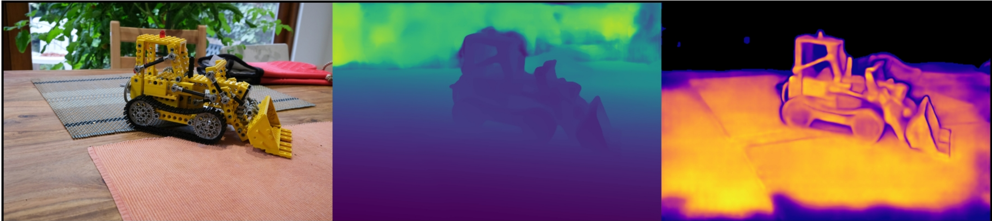
kitchen: VGGT | num_images=100 Original | Depth (max=2.43) | Confidence (max=30.80)
