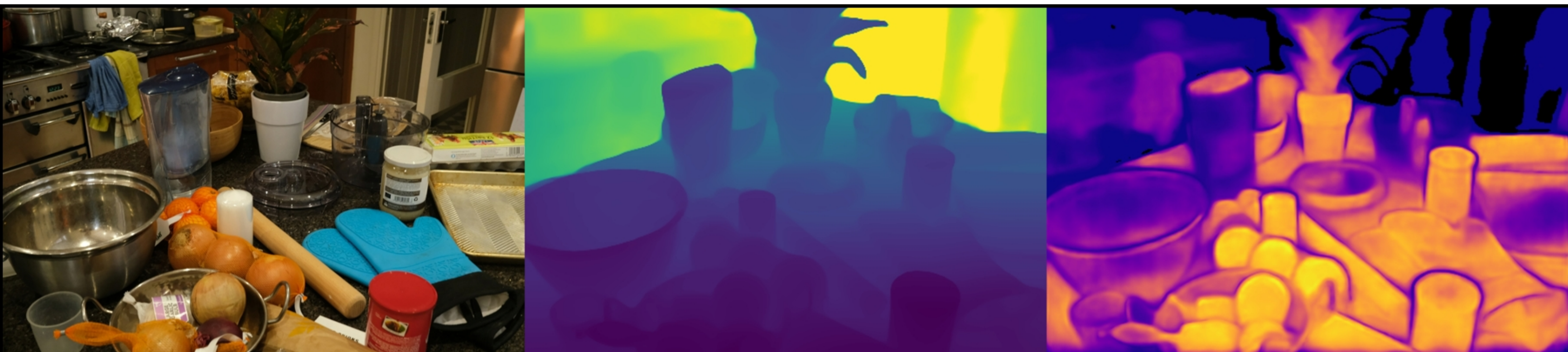
counter: VGGT | num_images=20 Original | Depth (max=2.77) | Confidence (max=15.05)
