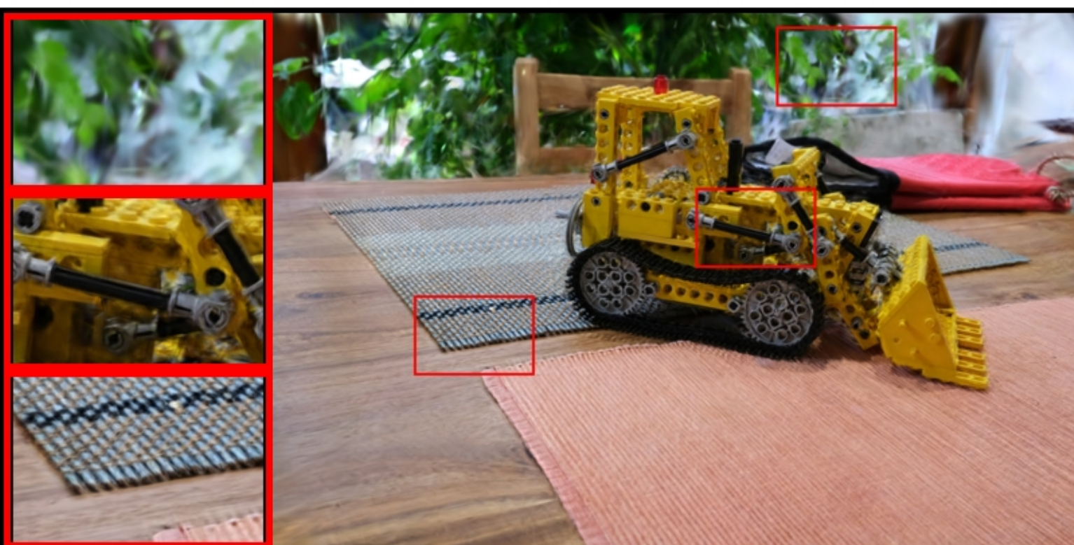
kitchen: VGGT | num_images=40 PSNR: 17.73 | LPIPS: 0.2962 | SSIM: 0.3957
