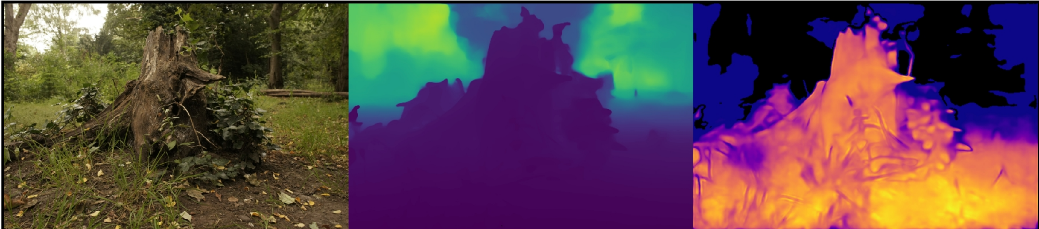
stump: VGGT | num_images=100 Original | Depth (max=6.21) | Confidence (max=3.47)
