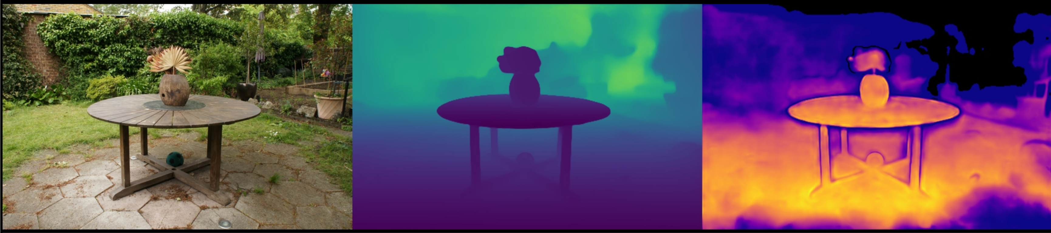
garden: VGGT | num_images=40 Original | Depth (max=2.46) | Confidence (max=5.54)
