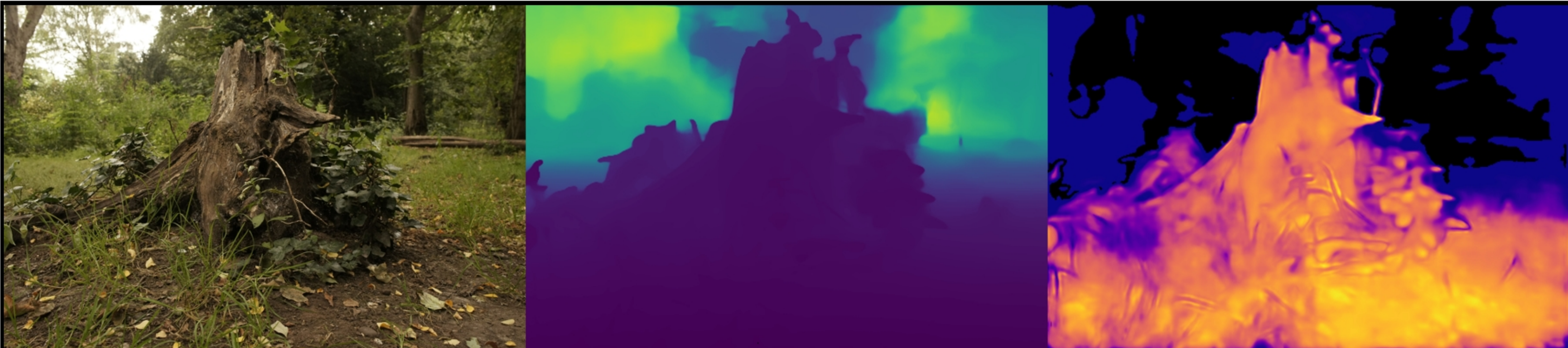
stump: VGGT | num_images=40 Original | Depth (max=5.96) | Confidence (max=2.36)
