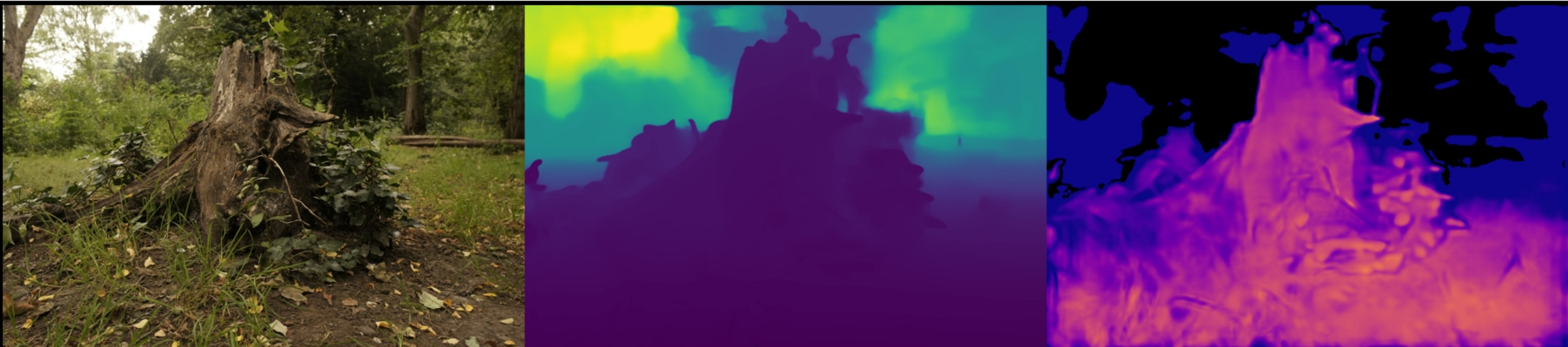
stump: VGGT | num_images=20 Original | Depth (max=5.38) | Confidence (max=1.70)
