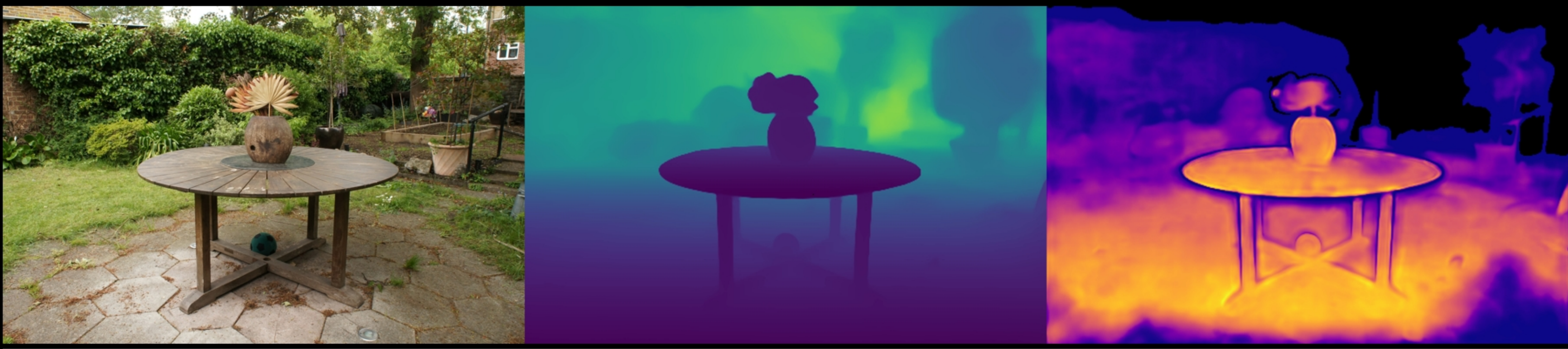
garden: VGGT | num_images=20 Original | Depth (max=2.67) | Confidence (max=5.47)
