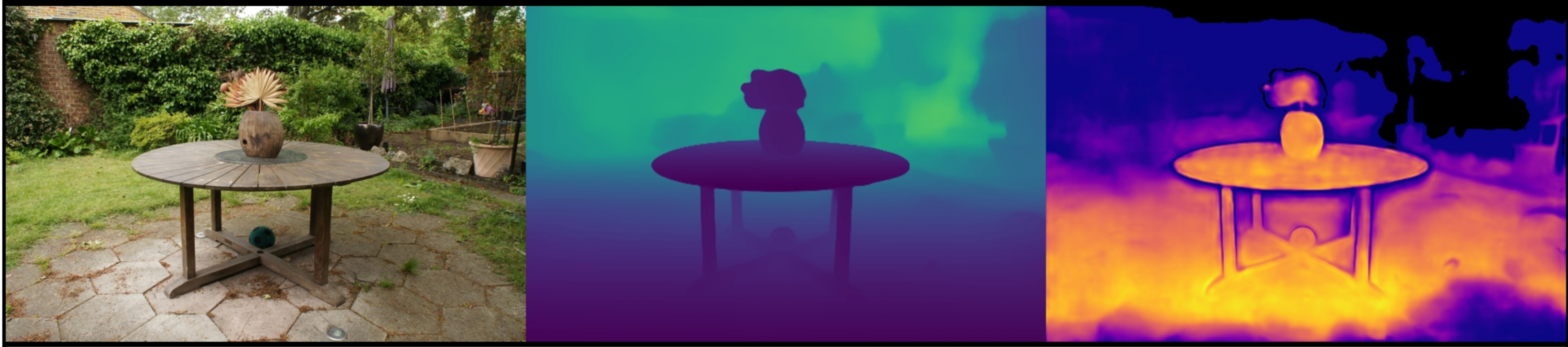
garden: VGGT | num_images=100 Original | Depth (max=2.46) | Confidence (max=6.23)
